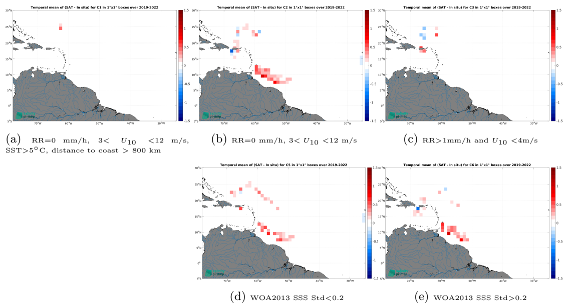
Figure 14: Temporal mean gridded over spatial boxes of size 1^\circ \times 1^\circ of \Delta SSS (SMAP SSS L3 v6 - 8-Day running (RSS) - Saildrone) for 5 different subdatasets corresponding to:RR=0 mm/h, 3 < U_{10} < 12 m/s, SST >5^\circ\text{C} , distance to coast > 800 km (a), RR=0 mm/h, 3 < U_{10} < 12 m/s (b), RR >1 mm/h and U_{10} < 4 m/s (c), WOA2013 SSS Std <0.2 (d), WOA2013 SSS Std >0.2 (e).
