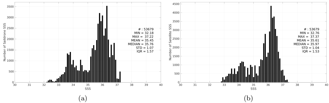
Figure 3: Histograms of SSS from Saildrone (a) and SMAP SSS L3 v6 - 8-Day running (RSS) (b) considering all match-up pairs per bins of 0.1 over the Amazon and Orinoco river plumes Pi-MEP region and for the full satellite product period.
