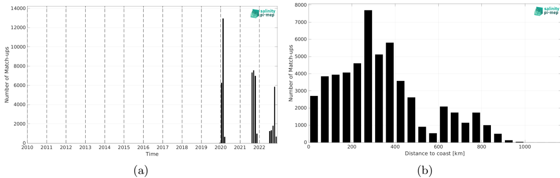
Figure 2: Number of match-ups between Saildrone and SMAP SSS L3 v6 - 8-Day running (RSS) SSS as a function of time (a) and as function of the distance to coast (b) over the Amazon and Orinoco river plumes Pi-MEP region and for the full satellite product period.
