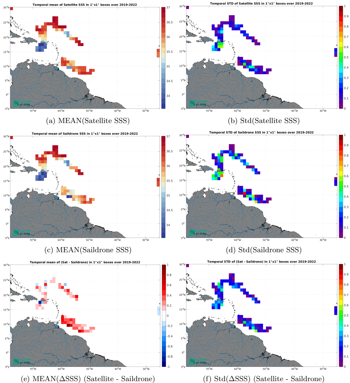
Figure 7: Temporal mean (left) and Std (right) of SSS from SMAP SSS L3 v6 - 8-Day running (RSS) (top), Saildrone (middle), and of \Delta SSS (Satellite - Saildrone). Only match-up pairs are used to generate these maps.
