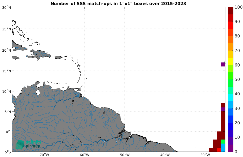
Figure 5: Number of SSS match-ups between TSG (Polarstern) SSS and the SMAP SSS L3 v6 - Monthly (RSS) SSS product for the Amazon and Orinoco river plumes Pi-MEP region over 1^\circ \times 1^\circ boxes and for the full satellite product period.
