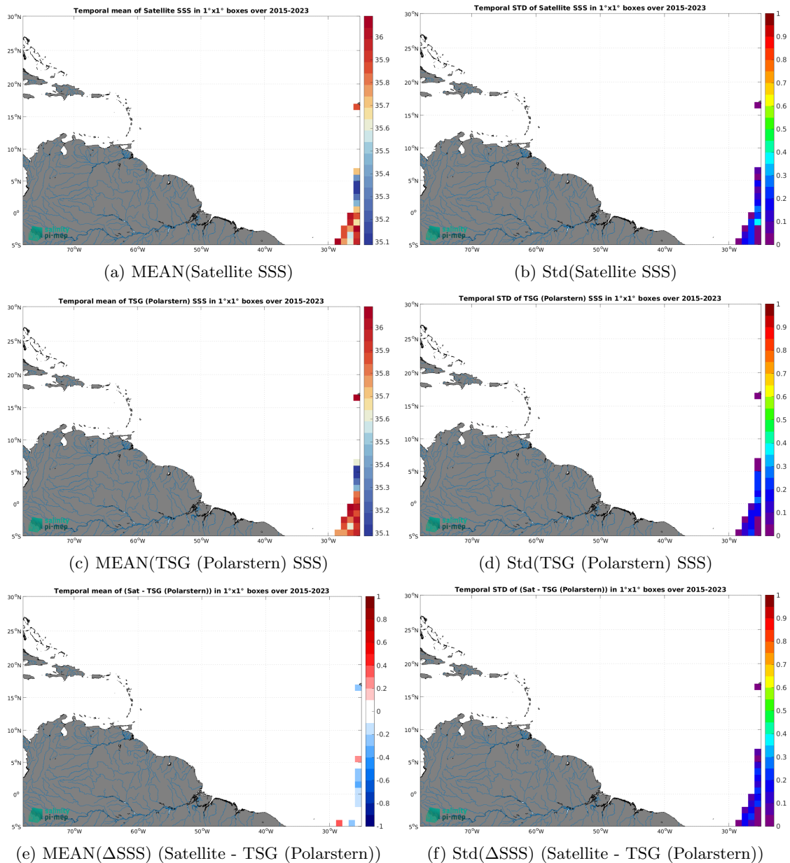
Figure 7: Temporal mean (left) and Std (right) of SSS from SMAP SSS L3 v6 - Monthly (RSS) (top), TSG (Polarstern) (middle), and of \Delta SSS (Satellite - TSG (Polarstern)). Only match-up pairs are used to generate these maps.
