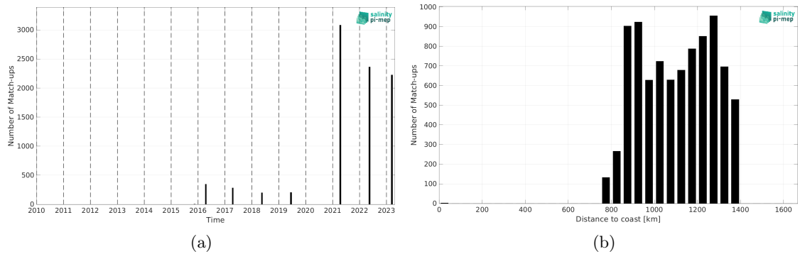
Figure 2: Number of match-ups between TSG (Polarstern) and SMAP SSS L3 v6 - Monthly (RSS) SSS as a function of time (a) and as function of the distance to coast (b) over the Amazon and Orinoco river plumes Pi-MEP region and for the full satellite product period.
