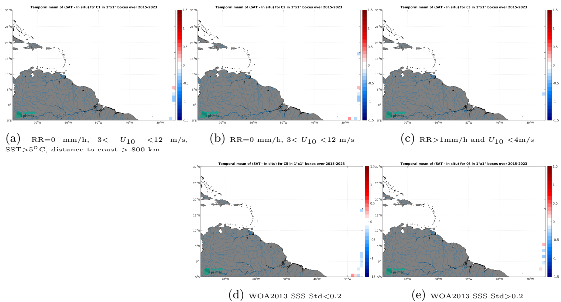
Figure 14: Temporal mean gridded over spatial boxes of size 1^\circ \times 1^\circ of \Delta SSS (SMAP SSS L3 v6 - Monthly (RSS) - TSG (Polarstern)) for 5 different subdatasets corresponding to:RR=0 mm/h, 3 < U_{10} < 12 m/s, SST >5^\circ\text{C} , distance to coast > 800 km (a), RR=0 mm/h, 3 < U_{10} < 12 m/s (b), RR >1 mm/h and U_{10} < 4 m/s (c), WOA2013 SSS Std <0.2 (d), WOA2013 SSS Std >0.2 (e).
