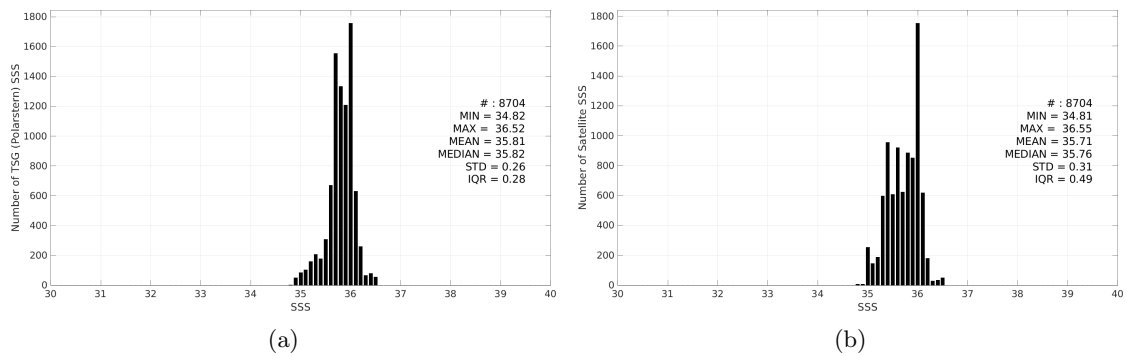
Figure 3: Histograms of SSS from TSG (Polarstern) (a) and SMAP SSS L3 v6 - Monthly (RSS) (b) considering all match-up pairs per bins of 0.1 over the Amazon and Orinoco river plumes Pi-MEP region and for the full satellite product period.
