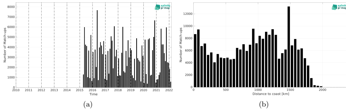
Figure 2: Number of match-ups between TSG (LEGOS-DM) and SMAP SSS L3 v6 - Monthly (RSS) SSS as a function of time (a) and as function of the distance to coast (b) over the Amazon and Orinoco river plumes Pi-MEP region and for the full satellite product period.
