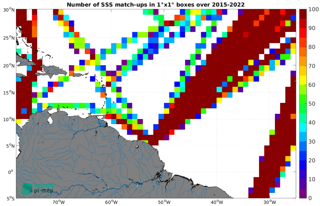
Figure 5: Number of SSS match-ups between TSG (LEGOS-DM) SSS and the SMAP SSS L3 v6 - Monthly (RSS) SSS product for the Amazon and Orinoco river plumes Pi-MEP region over 1^\circ \times 1^\circ boxes and for the full satellite product period.
