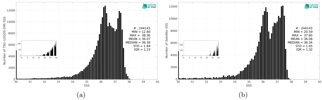
Figure 3: Histograms of SSS from TSG (LEGOS-DM) (a) and SMAP SSS L3 v6 - Monthly (RSS) (b) considering all match-up pairs per bins of 0.1 over the Amazon and Orinoco river plumes Pi-MEP region and for the full satellite product period.
