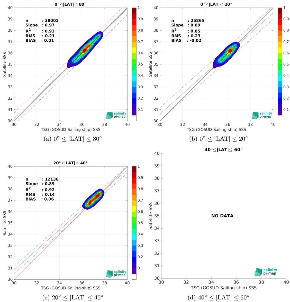
Figure 10: Contour maps of the concentration of SMAP SSS L3 v6 - Monthly (RSS) SSS (y-axis) versus TSG (GOSUD-Sailing-ship) SSS (x-axis) at match-up pairs for different latitude bands. For each plot, the red line shows x=y . The black thin and dashed lines indicate a linear fit through the data cloud and the \pm 95\% confidence levels, respectively. The number match-up pairs n , the slope and R^2 coefficient of the linear fit, the root mean square (RMS) and the mean bias between satellite and in situ data are indicated for each latitude band in each plots.
