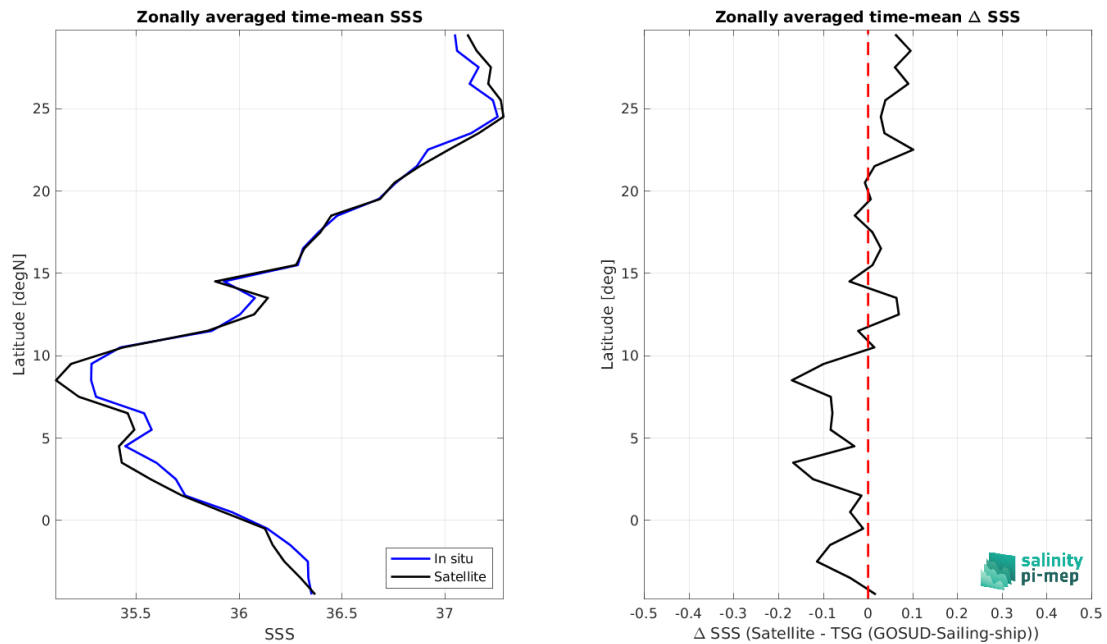
Figure 9: Left panel: Zonal mean SSS from SMAP SSS L3 v6 - Monthly (RSS) satellite product (black) and from TSG (GOSUD-Sailing-ship) (blue). Right panel: Zonal mean of \Delta SSS (Satellite - TSG (GOSUD-Sailing-ship)) for all the collected Pi-MEP match-up pairs estimated over the full satellite product period.
