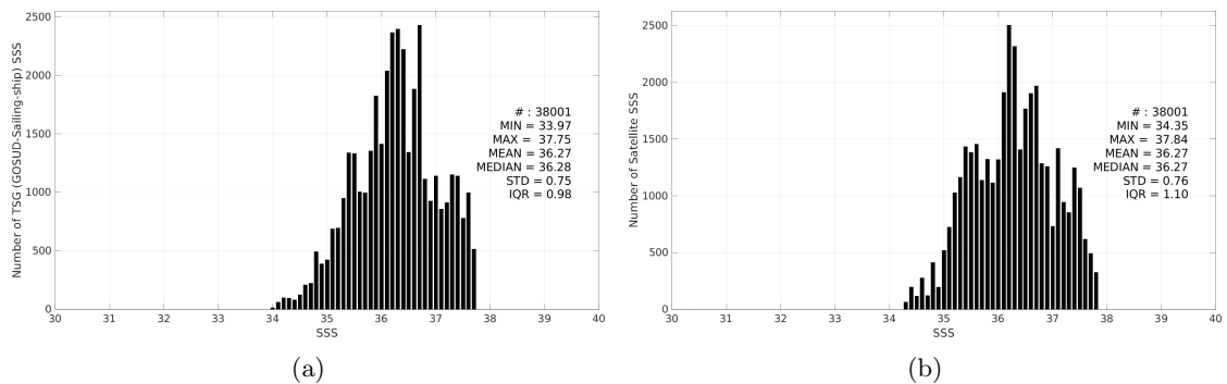
Figure 3: Histograms of SSS from TSG (GOSUD-Sailing-ship) (a) and SMAP SSS L3 v6 - Monthly (RSS) (b) considering all match-up pairs per bins of 0.1 over the Amazon and Orinoco river plumes Pi-MEP region and for the full satellite product period.
