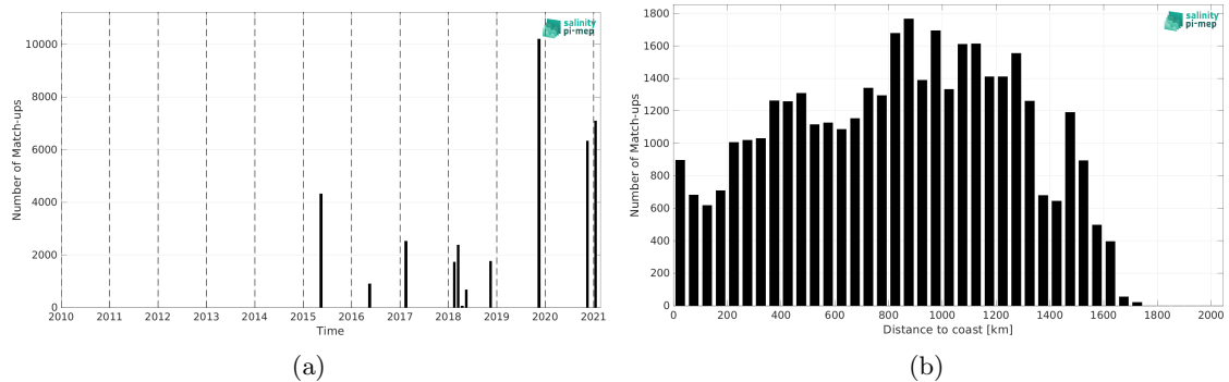
Figure 2: Number of match-ups between TSG (GOSUD-Sailing-ship) and SMAP SSS L3 v6 - Monthly (RSS) SSS as a function of time (a) and as function of the distance to coast (b) over the Amazon and Orinoco river plumes Pi-MEP region and for the full satellite product period.
