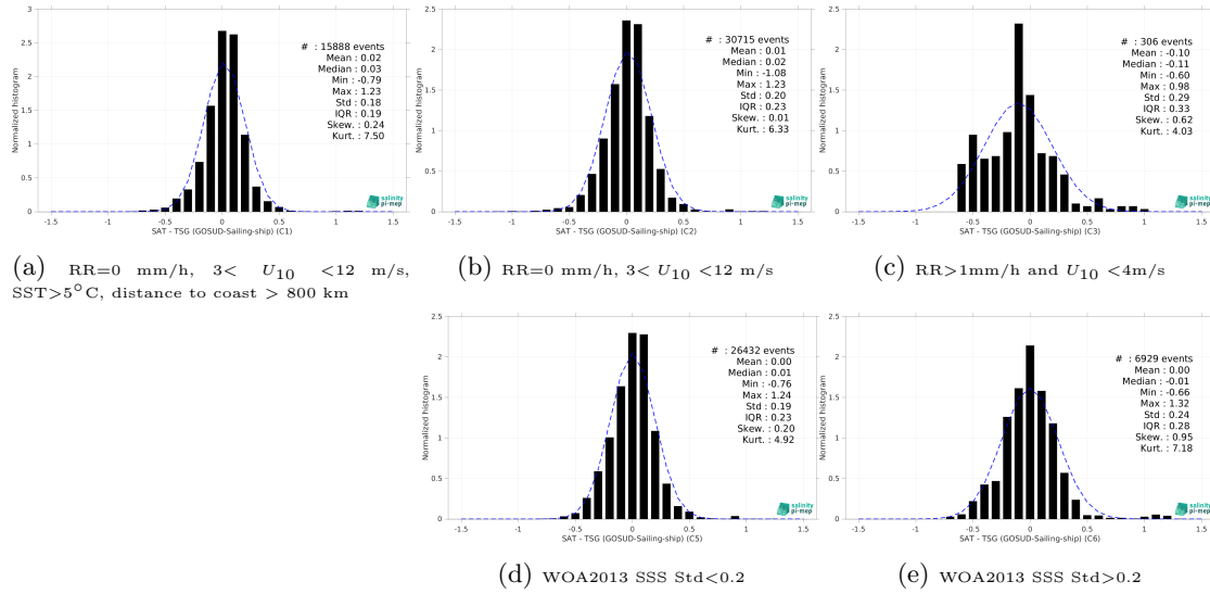
Figure 15: Normalized histogram of \Delta SSS (SMAP SSS L3 v6 - Monthly (RSS) - TSG (GOSUD-Sailing-ship)) for 5 different subdatasets corresponding to: RR=0 mm/h, 3 < U_{10} < 12 m/s, SST > 5°C, distance to coast > 800 km (a), RR=0 mm/h, 3 < U_{10} < 12 m/s (b), RR > 1mm/h and U_{10} < 4 m/s (c), WOA2013 SSS Std < 0.2 (d), WOA2013 SSS Std > 0.2 (e).
