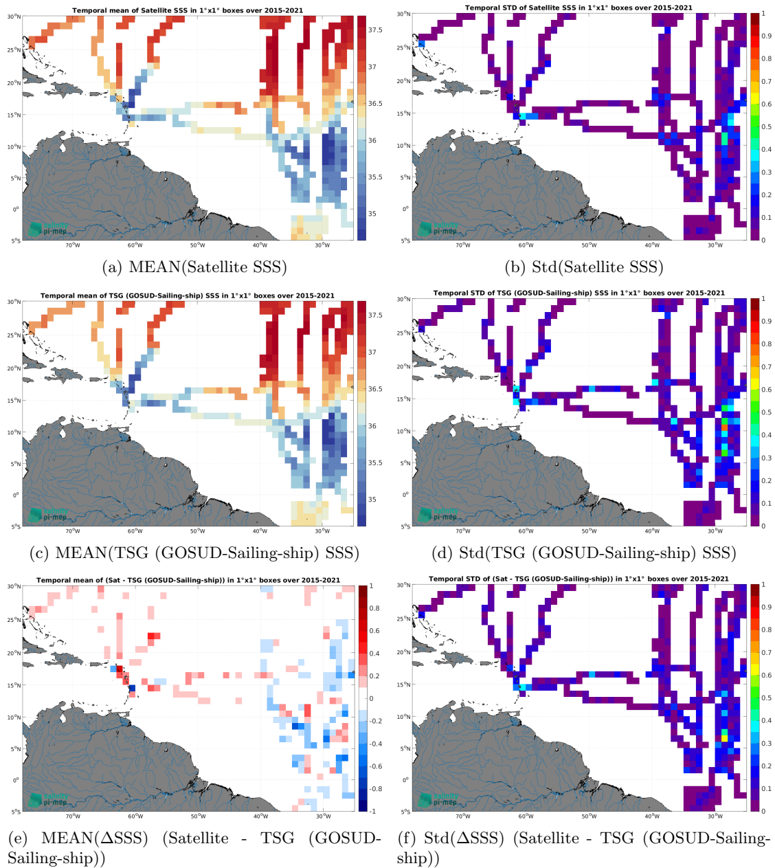
Figure 7: Temporal mean (left) and Std (right) of SSS from SMAP SSS L3 v6 - Monthly (RSS) (top), TSG (GOSUD-Sailing-ship) (middle), and of \Delta SSS (Satellite - TSG (GOSUD-Sailing-ship)). Only match-up pairs are used to generate these maps.
