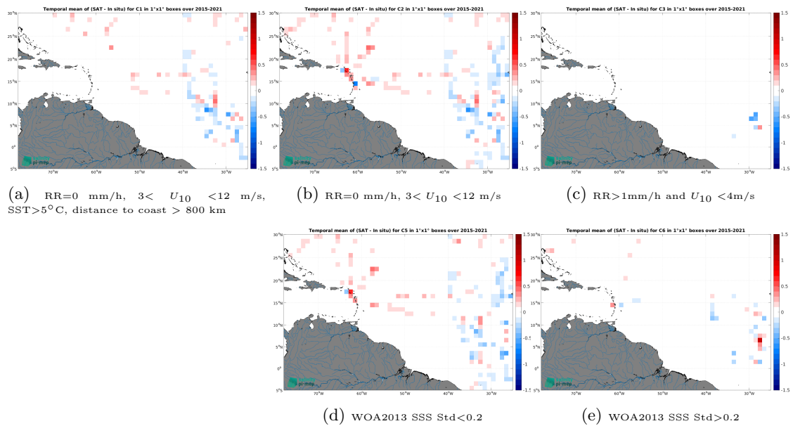
Figure 14: Temporal mean gridded over spatial boxes of size 1^\circ \times 1^\circ of \Delta SSS (SMAP SSS L3 v6 - Monthly (RSS) - TSG (GOSUD-Sailing-ship)) for 5 different subdatasets corresponding to:RR=0 mm/h, 3 < U_{10} < 12 m/s, SST >5^\circ\text{C} , distance to coast > 800 km (a), RR=0 mm/h, 3 < U_{10} < 12 m/s (b), RR >1 mm/h and U_{10} < 4 m/s (c), WOA2013 SSS Std <0.2 (d), WOA2013 SSS Std >0.2 (e).
