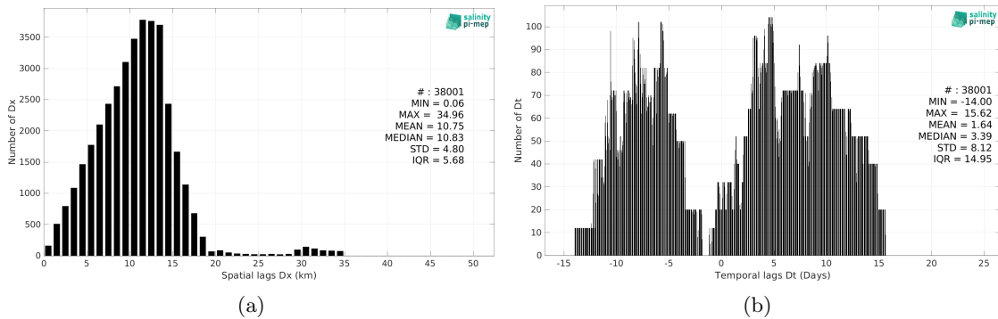
Figure 6: Histograms of the spatial (a) and temporal (b) lags between the location/time of the TSG (GOSUD-Sailing-ship) measurement and the date of the corresponding SMAP SSS L3 v6 - Monthly (RSS) SSS pixel.
