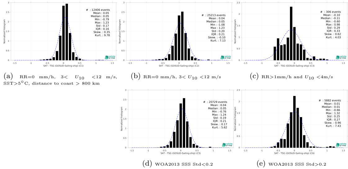
Figure 15: Normalized histogram of \Delta SSS (SMAP SSS L3 v6 - Monthly (RSS) - TSG (GOSUD-Sailing-ship)) for 5 different subdatasets corresponding to: RR=0 mm/h, 3 < U_{10} < 12 m/s, SST >5^{\circ} C, distance to coast > 800 km (a), RR=0 mm/h, 3 < U_{10} < 12 m/s (b), RR >1 mm/h and U_{10} < 4 m/s (c), WOA2013 SSS Std <0.2 (d), WOA2013 SSS Std >0.2 (e).
