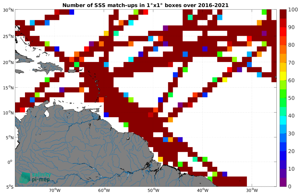
Figure 5: Number of SSS match-ups between TSG (GOSUD-Research-vessel) SSS and the SMAP SSS L3 v6 - Monthly (RSS) SSS product for the Amazon and Orinoco river plumes Pi-MEP region over 1^{\circ} \times 1^{\circ} boxes and for the full satellite product period.
