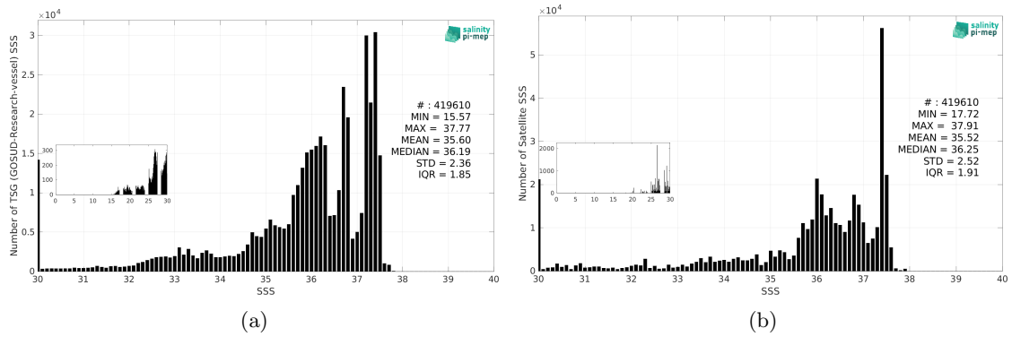
Figure 3: Histograms of SSS from TSG (GOSUD-Research-vessel) (a) and SMAP SSS L3 v6 - Monthly (RSS) (b) considering all match-up pairs per bins of 0.1 over the Amazon and Orinoco river plumes Pi-MEP region and for the full satellite product period.
