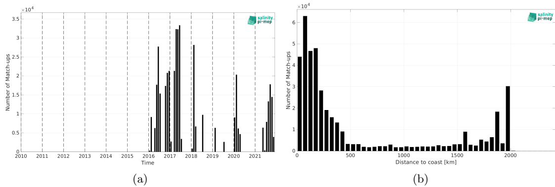
Figure 2: Number of match-ups between TSG (GOSUD-Research-vessel) and SMAP SSS L3 v6 - Monthly (RSS) SSS as a function of time (a) and as function of the distance to coast (b) over the Amazon and Orinoco river plumes Pi-MEP region and for the full satellite product period.
