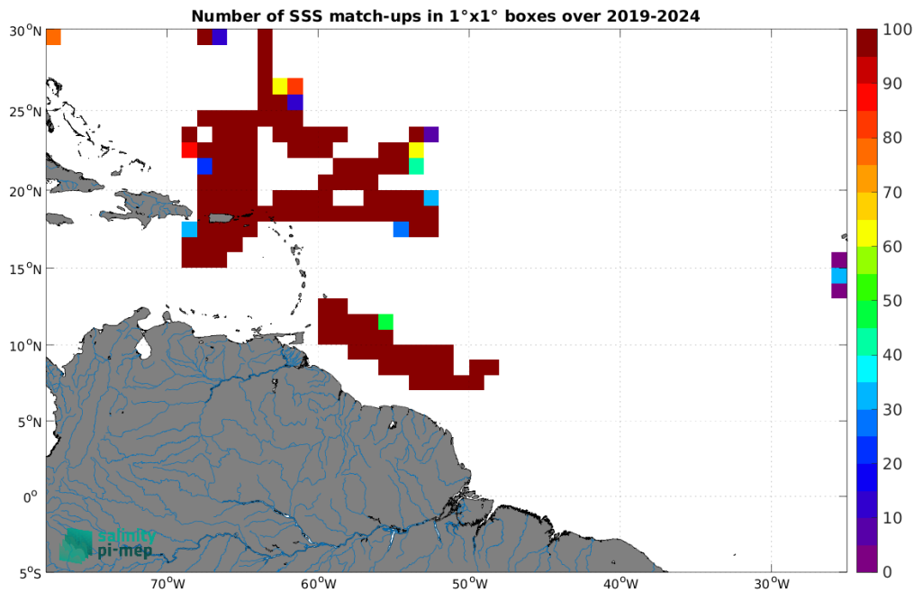
Figure 5: Number of SSS match-ups between Saildrone SSS and the SMAP SSS L3 v6 - Monthly (RSS) SSS product for the Amazon and Orinoco river plumes Pi-MEP region over 1°x1° boxes and for the full satellite product period.
