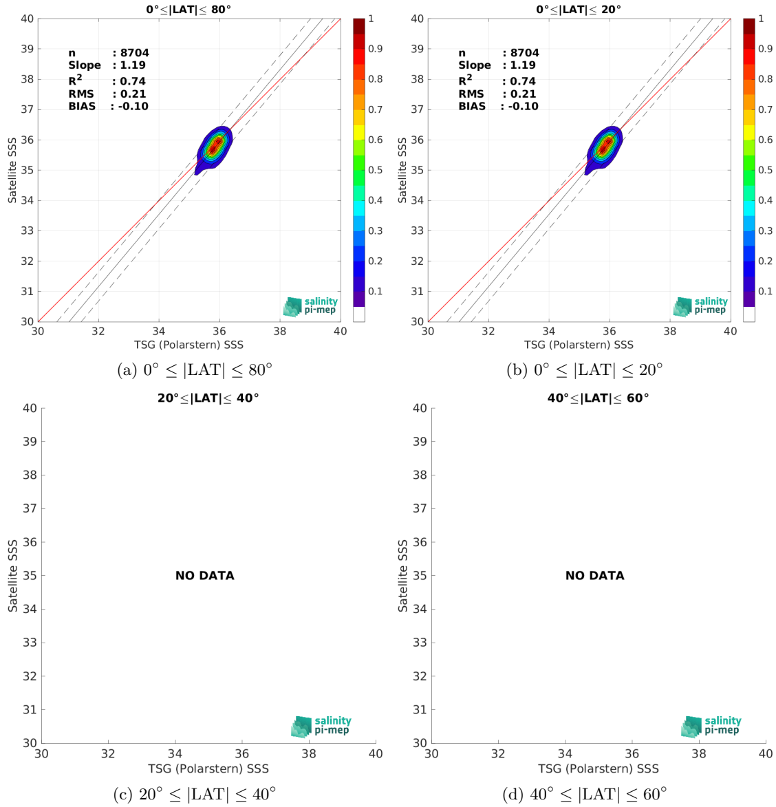
Figure 10: Contour maps of the concentration of SMAP SSS L3 v5.3 - 8-Day running (RSS) SSS (y-axis) versus TSG (Polarstern) SSS (x-axis) at match-up pairs for different latitude bands. For each plot, the red line shows x=y . The black thin and dashed lines indicate a linear fit through the data cloud and the \pm 95\% confidence levels, respectively. The number match-up pairs n , the slope and R^2 coefficient of the linear fit, the root mean square (RMS) and the mean bias between satellite and in situ data are indicated for each latitude band in each plots.
