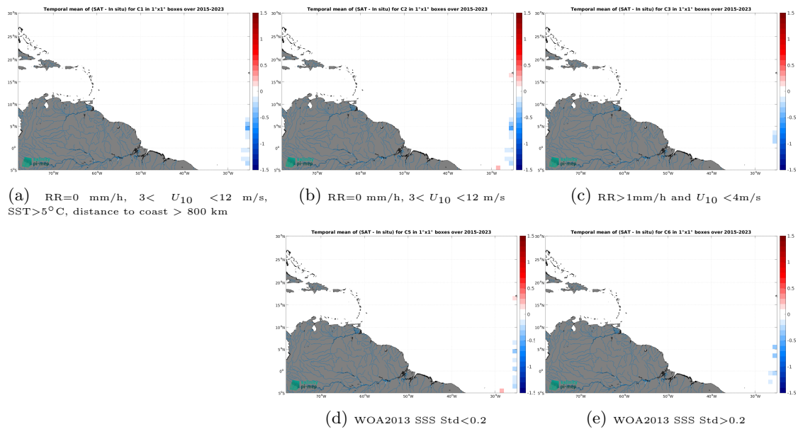
Figure 14: Temporal mean gridded over spatial boxes of size 1^\circ \times 1^\circ of \Delta SSS (SMAP SSS L3 v5.3 - 8-Day running (RSS) - TSG (Polarstern)) for 5 different subdatasets corresponding to: RR=0 mm/h, 3 < U_{10} < 12 m/s, SST > 5°C, distance to coast > 800 km (a), RR=0 mm/h, 3 < U_{10} < 12 m/s (b), RR > 1mm/h and U_{10} < 4 m/s (c), WOA2013 SSS Std < 0.2 (d), WOA2013 SSS Std > 0.2 (e).
