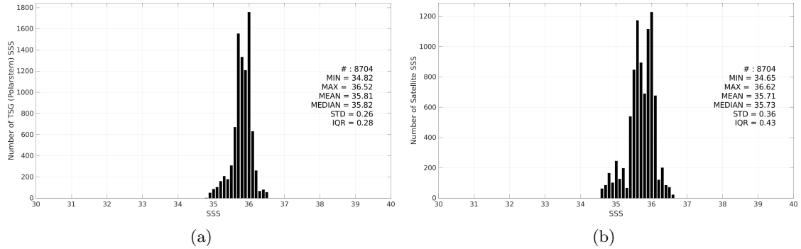
Figure 3: Histograms of SSS from TSG (Polarstern) (a) and SMAP SSS L3 v5.3 - 8-Day running (RSS) (b) considering all match-up pairs per bins of 0.1 over the Amazon and Orinoco river plumes Pi-MEP region and for the full satellite product period.
