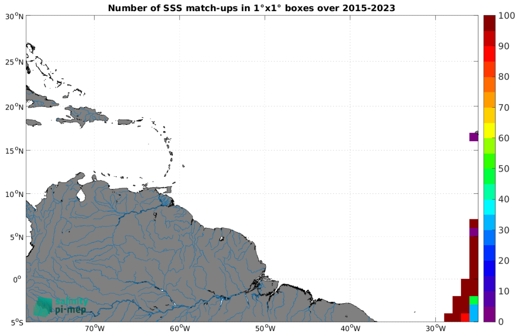
Figure 5: Number of SSS match-ups between TSG (Polarstern) SSS and the SMAP SSS L3 v5.3 - 8-Day running (RSS) SSS product for the Amazon and Orinoco river plumes Pi-MEP region over 1^\circ \times 1^\circ boxes and for the full satellite product period.
