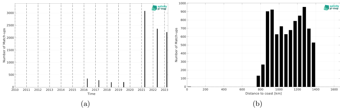
Figure 2: Number of match-ups between TSG (Polarstern) and SMAP SSS L3 v5.3 - 8-Day running (RSS) SSS as a function of time (a) and as function of the distance to coast (b) over the Amazon and Orinoco river plumes Pi-MEP region and for the full satellite product period.
