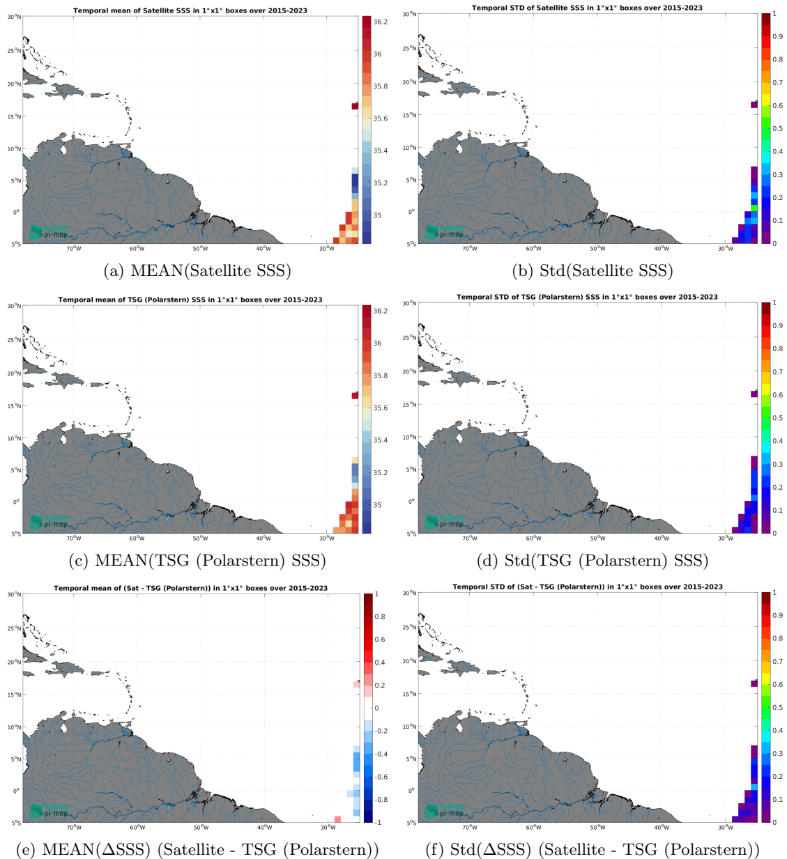
Figure 7: Temporal mean (left) and Std (right) of SSS from SMAP SSS L3 v5.3 - 8-Day running (RSS) (top), TSG (Polarstern) (middle), and of \Delta SSS (Satellite - TSG (Polarstern)). Only match-up pairs are used to generate these maps.
