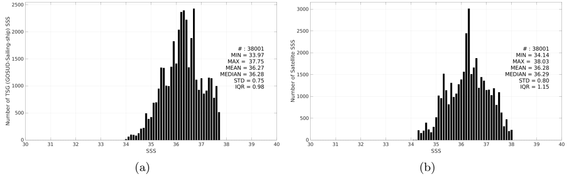
Figure 3: Histograms of SSS from TSG (GOSUD-Sailing-ship) (a) and SMAP SSS L3 v5.3 - 8-Day running (RSS) (b) considering all match-up pairs per bins of 0.1 over the Amazon and Orinoco river plumes Pi-MEP region and for the full satellite product period.
