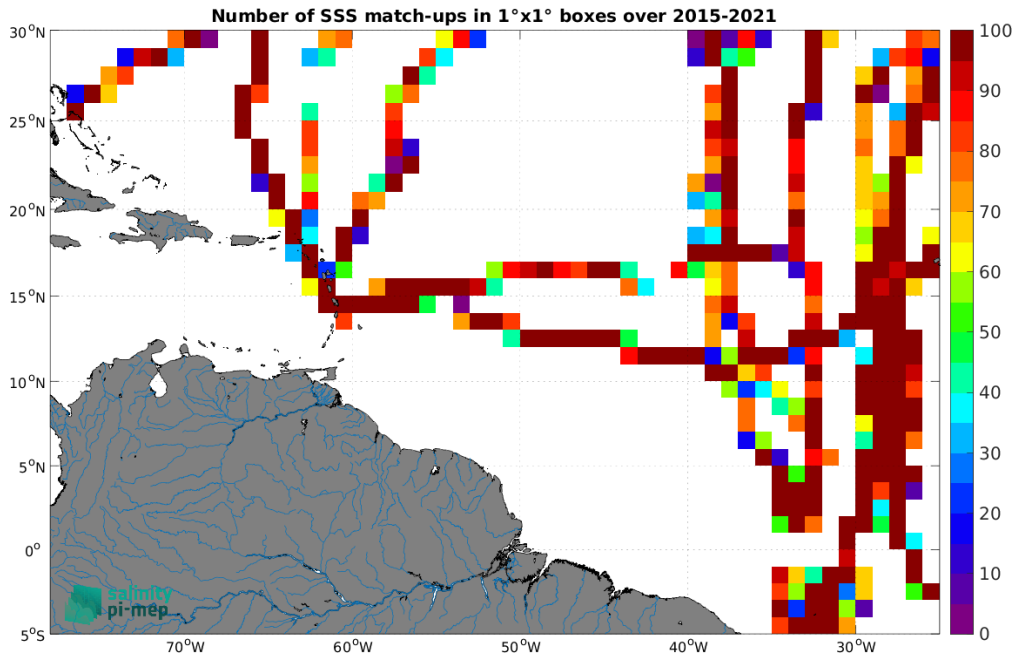
Figure 5: Number of SSS match-ups between TSG (GOSUD-Sailing-ship) SSS and the SMAP SSS L3 v5.3 - 8-Day running (RSS) SSS product for the Amazon and Orinoco river plumes Pi-MEP region over 1^\circ \times 1^\circ boxes and for the full satellite product period.
