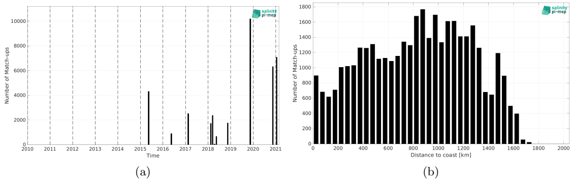
Figure 2: Number of match-ups between TSG (GOSUD-Sailing-ship) and SMAP SSS L3 v5.3 - 8-Day running (RSS) SSS as a function of time (a) and as function of the distance to coast (b) over the Amazon and Orinoco river plumes Pi-MEP region and for the full satellite product period.
