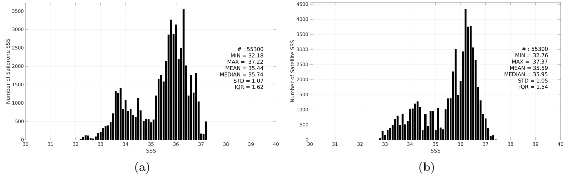
Figure 3: Histograms of SSS from Saildrone (a) and SMAP SSS L3 v5.3 - 8-Day running (RSS) (b) considering all match-up pairs per bins of 0.1 over the Amazon and Orinoco river plumes Pi-MEP region and for the full satellite product period.
