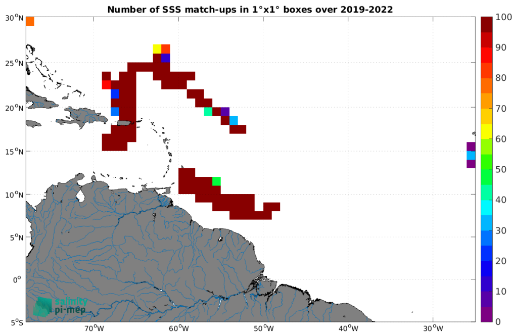
Figure 5: Number of SSS match-ups between Saildrone SSS and the SMAP SSS L3 v5.3 - 8-Day running (RSS) SSS product for the Amazon and Orinoco river plumes Pi-MEP region over 1^\circ \times 1^\circ boxes and for the full satellite product period.
