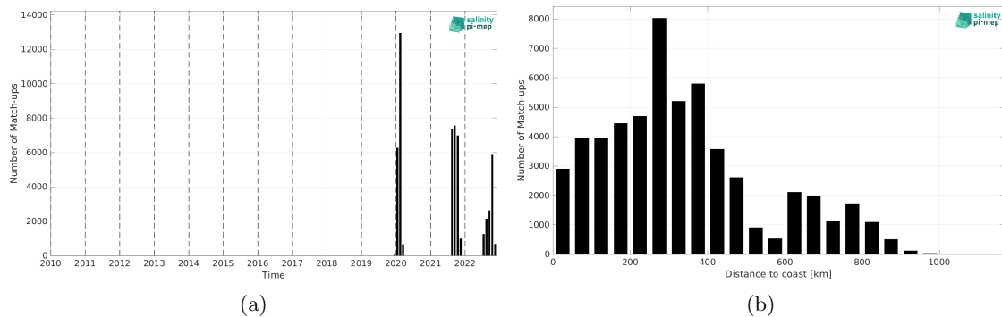
Figure 2: Number of match-ups between Saildrone and SMAP SSS L3 v5.3 - 8-Day running (RSS) SSS as a function of time (a) and as function of the distance to coast (b) over the Amazon and Orinoco river plumes Pi-MEP region and for the full satellite product period.
