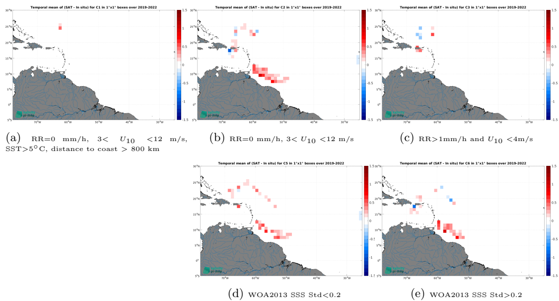
Figure 14: Temporal mean gridded over spatial boxes of size 1^\circ \times 1^\circ of \Delta SSS (SMAP SSS L3 v5.3 - 8-Day running (RSS) - Saildrone) for 5 different subdatasets corresponding to:RR=0 mm/h, 3 < U_{10} < 12 m/s, SST >5^\circ\text{C} , distance to coast > 800 km (a), RR=0 mm/h, 3 < U_{10} < 12 m/s (b), RR >1 mm/h and U_{10} < 4 m/s (c), WOA2013 SSS Std <0.2 (d), WOA2013 SSS Std >0.2 (e).
