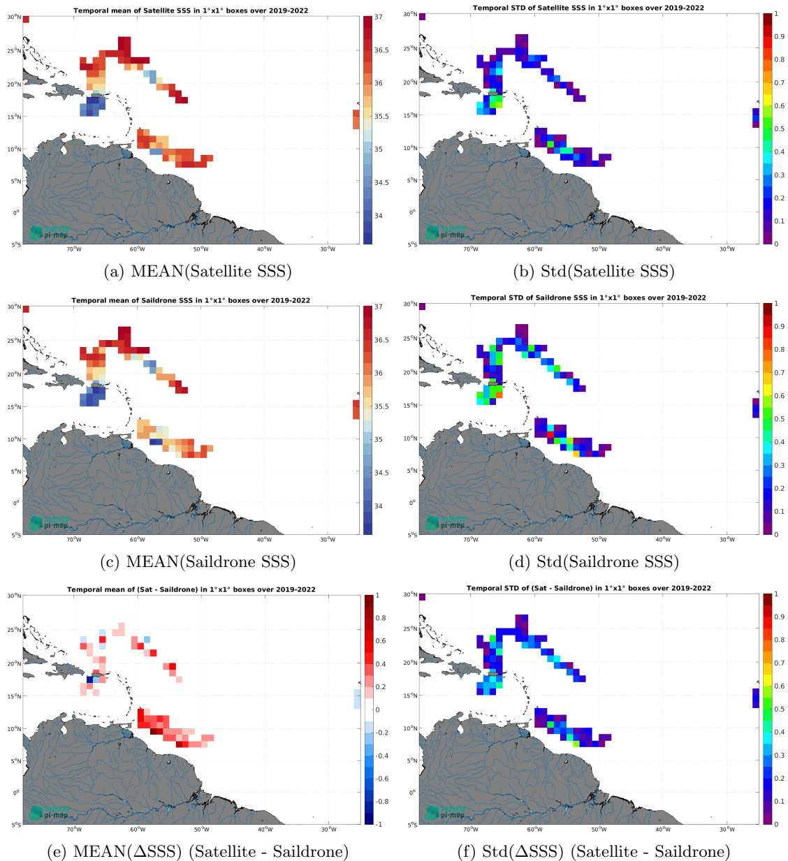
Figure 7: Temporal mean (left) and Std (right) of SSS from SMAP SSS L3 v5.3 - 8-Day running (RSS) (top), Saildrone (middle), and of \Delta SSS (Satellite - Saildrone). Only match-up pairs are used to generate these maps.
