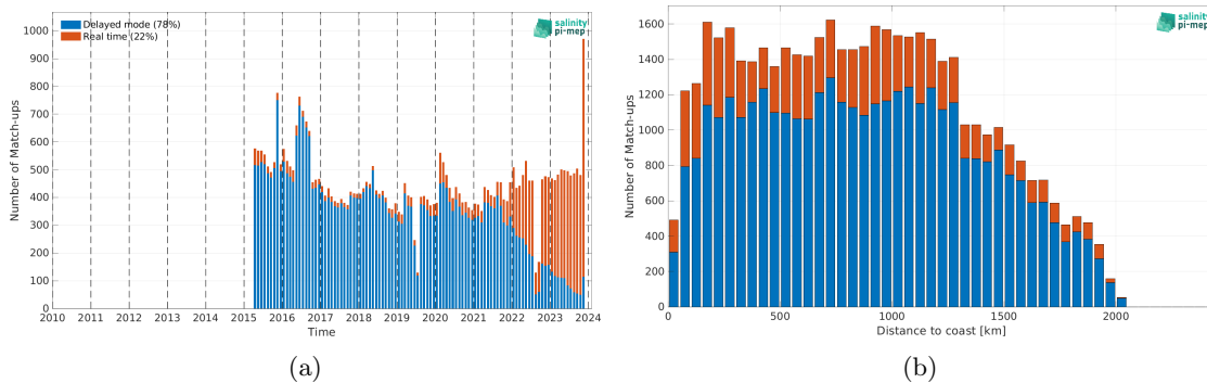
Figure 2: Number of match-ups between Argo and SMAP SSS L3 v5.3 - 8-Day running (RSS) SSS as a function of time (a) and as function of the distance to coast (b) over the Amazon and Orinoco river plumes Pi-MEP region and for the full satellite product period.
