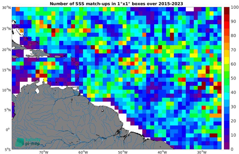
Figure 5: Number of SSS match-ups between Argo SSS and the SMAP SSS L3 v5.3 - 8-Day running (RSS) SSS product for the Amazon and Orinoco river plumes Pi-MEP region over 1^\circ \times 1^\circ boxes and for the full satellite product period.
