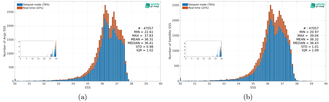
Figure 3: Histograms of SSS from Argo (a) and SMAP SSS L3 v5.3 - 8-Day running (RSS) (b) considering all match-up pairs per bins of 0.1 over the Amazon and Orinoco river plumes Pi-MEP region and for the full satellite product period.
