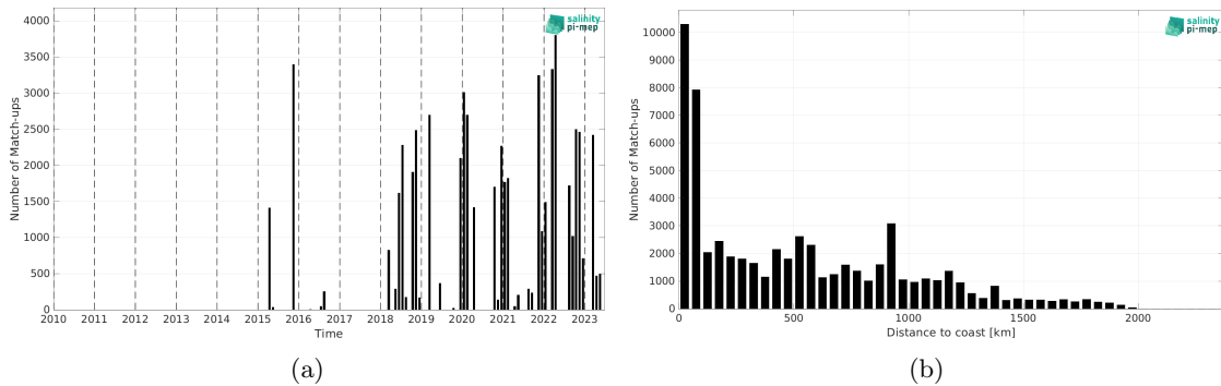
Figure 2: Number of match-ups between TSG (SAMOS) and SMAP SSS L3 v5.3 - Monthly (RSS) SSS as a function of time (a) and as function of the distance to coast (b) over the Amazon and Orinoco river plumes Pi-MEP region and for the full satellite product period.
