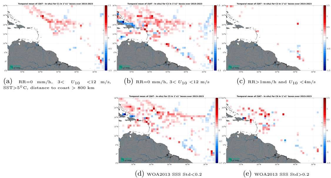
Figure 14: Temporal mean gridded over spatial boxes of size 1^\circ \times 1^\circ of \Delta SSS (SMAP SSS L3 v5.3 - Monthly (RSS) - TSG (SAMOS)) for 5 different subdatasets corresponding to:RR=0 mm/h, 3 < U_{10} < 12 m/s, SST >5^\circ\text{C} , distance to coast > 800 km (a), RR=0 mm/h, 3 < U_{10} < 12 m/s (b), RR >1 mm/h and U_{10} < 4 m/s (c), WOA2013 SSS Std <0.2 (d), WOA2013 SSS Std >0.2 (e).
