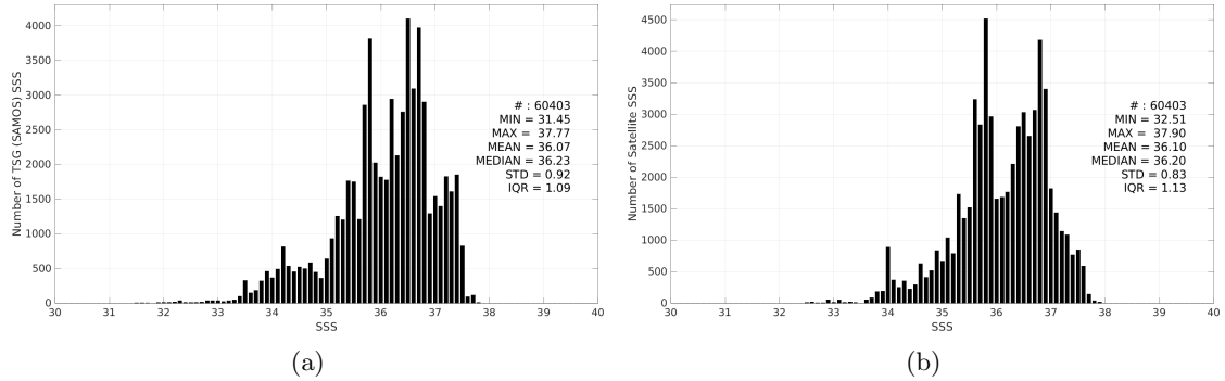
Figure 3: Histograms of SSS from TSG (SAMOS) (a) and SMAP SSS L3 v5.3 - Monthly (RSS) (b) considering all match-up pairs per bins of 0.1 over the Amazon and Orinoco river plumes Pi-MEP region and for the full satellite product period.
