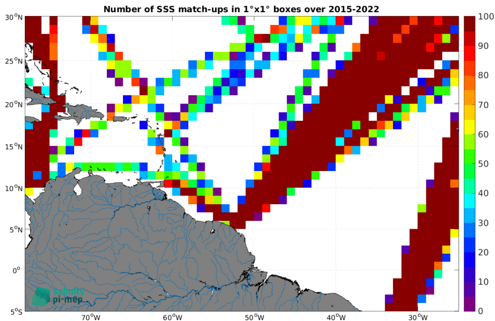
Figure 5: Number of SSS match-ups between TSG (LEGOS-DM) SSS and the SMAP SSS L3 v5.3 - Monthly (RSS) SSS product for the Amazon and Orinoco river plumes Pi-MEP region over 1^\circ \times 1^\circ boxes and for the full satellite product period.
