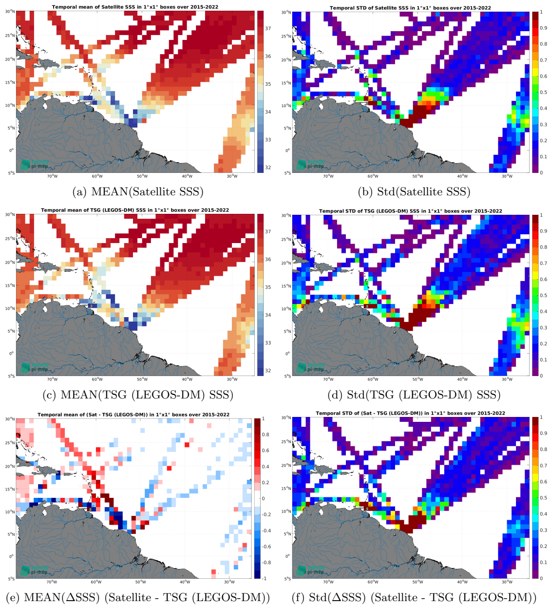
Figure 7: Temporal mean (left) and Std (right) of SSS from SMAP SSS L3 v5.3 - Monthly (RSS) (top), TSG (LEGOS-DM) (middle), and of \Delta SSS (Satellite - TSG (LEGOS-DM)). Only match-up pairs are used to generate these maps.
