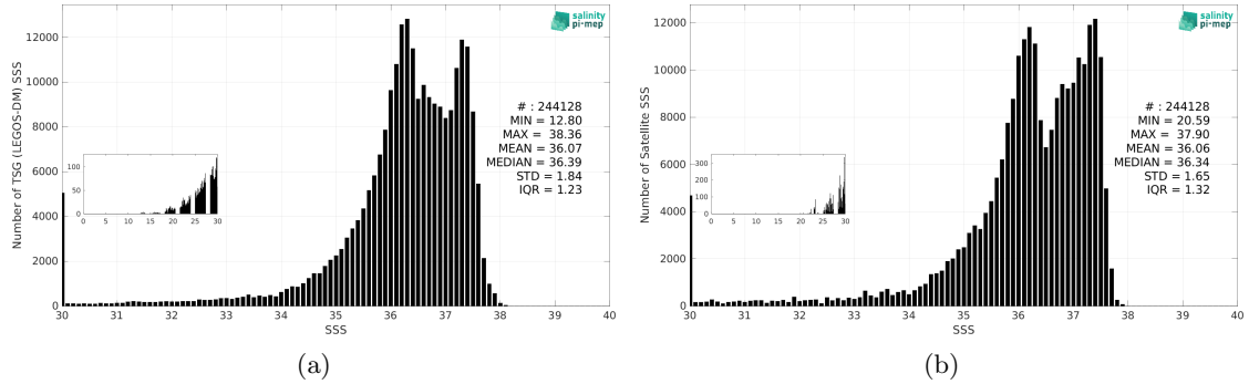
Figure 3: Histograms of SSS from TSG (LEGOS-DM) (a) and SMAP SSS L3 v5.3 - Monthly (RSS) (b) considering all match-up pairs per bins of 0.1 over the Amazon and Orinoco river plumes Pi-MEP region and for the full satellite product period.
