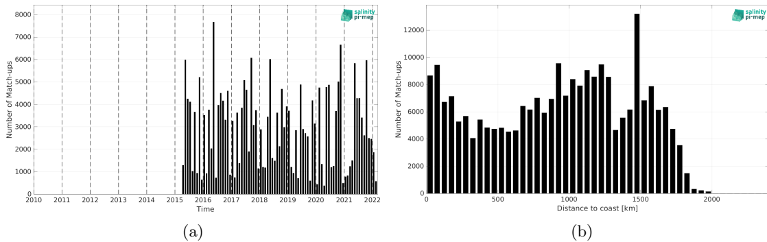
Figure 2: Number of match-ups between TSG (LEGOS-DM) and SMAP SSS L3 v5.3 - Monthly (RSS) SSS as a function of time (a) and as function of the distance to coast (b) over the Amazon and Orinoco river plumes Pi-MEP region and for the full satellite product period.
