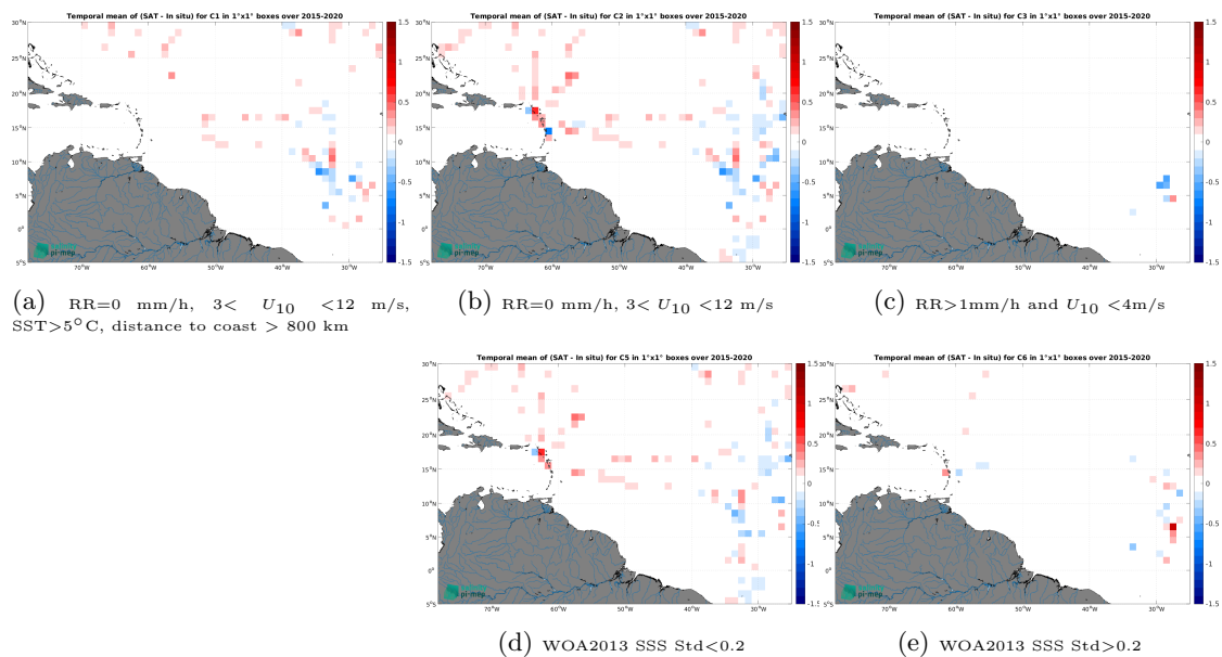
Figure 14: Temporal mean gridded over spatial boxes of size 1^\circ \times 1^\circ of \Delta\text{SSS} (SMAP SSS L3 v5.3 - Monthly (RSS) - TSG (GOSUD-Sailing-ship)) for 5 different subdatasets corresponding to:RR=0 mm/h, 3 < U_{10} < 12 m/s, SST >5^\circ\text{C} , distance to coast > 800 km (a), RR=0 mm/h, 3 < U_{10} < 12 m/s (b), RR >1 mm/h and U_{10} < 4 m/s (c), WOA2013 SSS Std <0.2 (d), WOA2013 SSS Std >0.2 (e).
