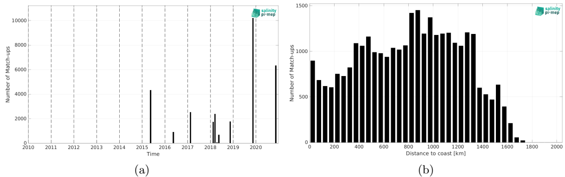
Figure 2: Number of match-ups between TSG (GOSUD-Sailing-ship) and SMAP SSS L3 v5.3 - Monthly (RSS) SSS as a function of time (a) and as function of the distance to coast (b) over the Amazon and Orinoco river plumes Pi-MEP region and for the full satellite product period.
