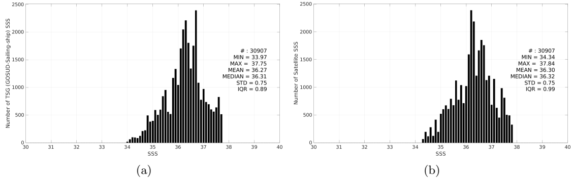
Figure 3: Histograms of SSS from TSG (GOSUD-Sailing-ship) (a) and SMAP SSS L3 v5.3 - Monthly (RSS) (b) considering all match-up pairs per bins of 0.1 over the Amazon and Orinoco river plumes Pi-MEP region and for the full satellite product period.
