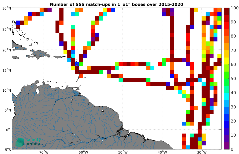
Figure 5: Number of SSS match-ups between TSG (GOSUD-Sailing-ship) SSS and the SMAP SSS L3 v5.3 - Monthly (RSS) SSS product for the Amazon and Orinoco river plumes Pi-MEP region over 1^\circ \times 1^\circ boxes and for the full satellite product period.
