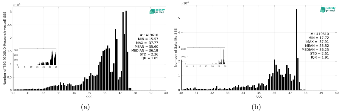
Figure 3: Histograms of SSS from TSG (GOSUD-Research-vessel) (a) and SMAP SSS L3 v5.3 - Monthly (RSS) (b) considering all match-up pairs per bins of 0.1 over the Amazon and Orinoco river plumes Pi-MEP region and for the full satellite product period.
