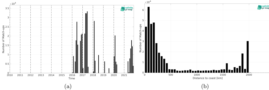
Figure 2: Number of match-ups between TSG (GOSUD-Research-vessel) and SMAP SSS L3 v5.3 - Monthly (RSS) SSS as a function of time (a) and as function of the distance to coast (b) over the Amazon and Orinoco river plumes Pi-MEP region and for the full satellite product period.
