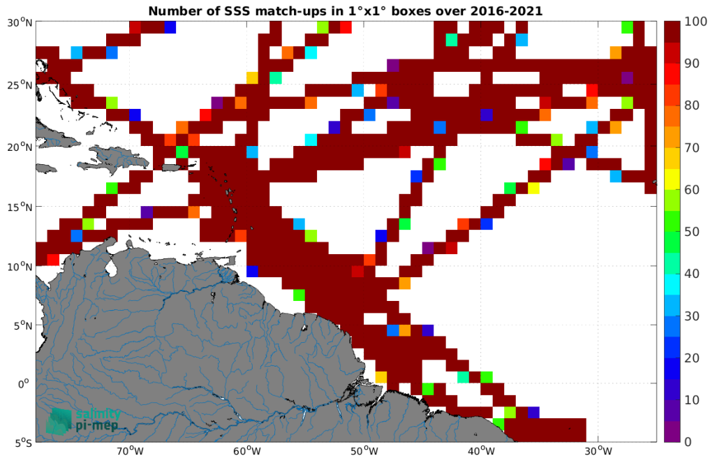
Figure 5: Number of SSS match-ups between TSG (GOSUD-Research-vessel) SSS and the SMAP SSS L3 v5.3 - Monthly (RSS) SSS product for the Amazon and Orinoco river plumes Pi-MEP region over 1^\circ \times 1^\circ boxes and for the full satellite product period.
