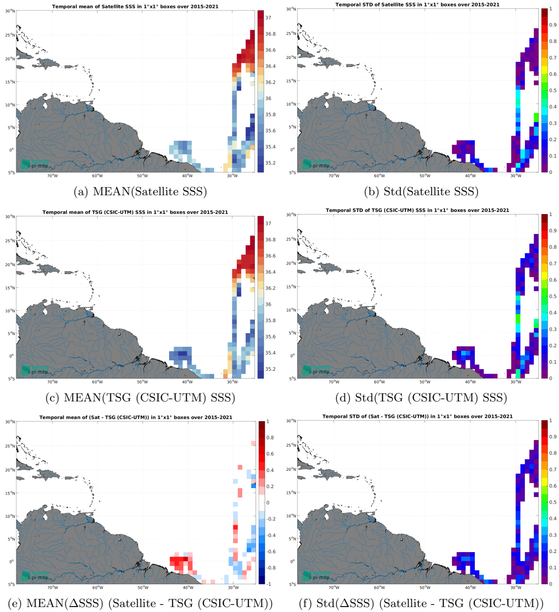
Figure 7: Temporal mean (left) and Std (right) of SSS from SMAP SSS L3 v5.3 - Monthly (RSS) (top), TSG (CSIC-UTM) (middle), and of \Delta SSS (Satellite - TSG (CSIC-UTM)). Only match-up pairs are used to generate these maps.
