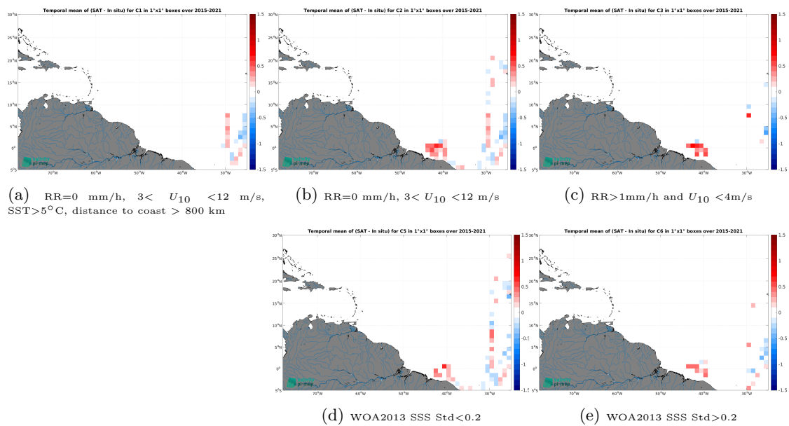
Figure 14: Temporal mean gridded over spatial boxes of size 1^\circ \times 1^\circ of \Delta SSS (SMAP SSS L3 v5.3 - Monthly (RSS) - TSG (CSIC-UTM)) for 5 different subdatasets corresponding to:RR=0 mm/h, 3 < U_{10} < 12 m/s, SST >5^\circ\text{C} , distance to coast > 800 km (a), RR=0 mm/h, 3 < U_{10} < 12 m/s (b), RR >1 mm/h and U_{10} < 4 m/s (c), WOA2013 SSS Std <0.2 (d), WOA2013 SSS Std >0.2 (e).
