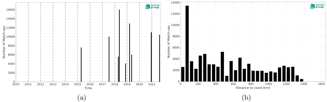
Figure 2: Number of match-ups between TSG (CSIC-UTM) and SMAP SSS L3 v5.3 - Monthly (RSS) SSS as a function of time (a) and as function of the distance to coast (b) over the Amazon and Orinoco river plumes Pi-MEP region and for the full satellite product period.
