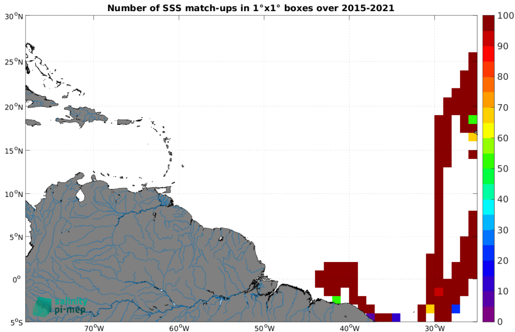
Figure 5: Number of SSS match-ups between TSG (CSIC-UTM) SSS and the SMAP SSS L3 v5.3 - Monthly (RSS) SSS product for the Amazon and Orinoco river plumes Pi-MEP region over 1°×1° boxes and for the full satellite product period.
