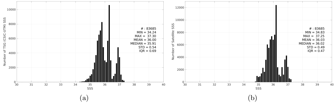
Figure 3: Histograms of SSS from TSG (CSIC-UTM) (a) and SMAP SSS L3 v5.3 - Monthly (RSS) (b) considering all match-up pairs per bins of 0.1 over the Amazon and Orinoco river plumes Pi-MEP region and for the full satellite product period.
