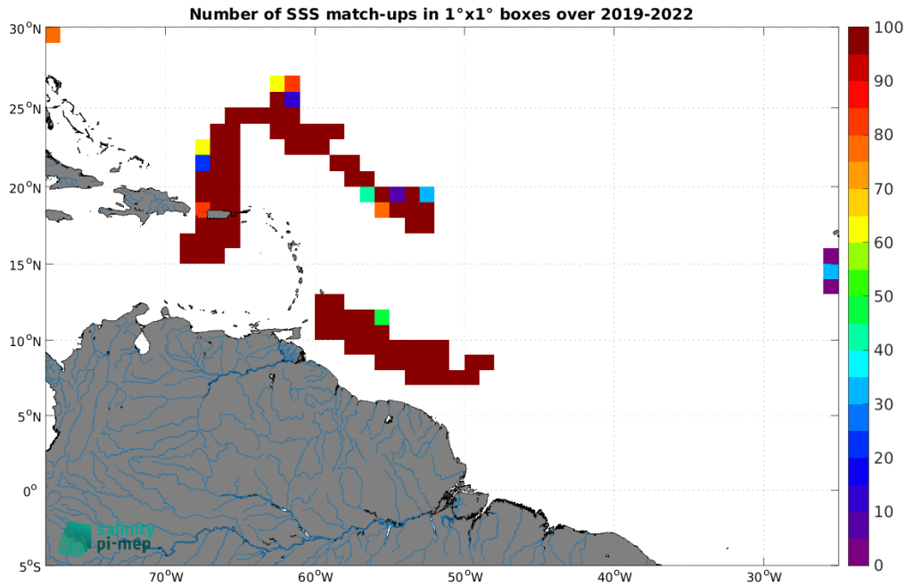
Figure 5: Number of SSS match-ups between Saildrone SSS and the SMAP SSS L3 v5.3 - Monthly (RSS) SSS product for the Amazon and Orinoco river plumes Pi-MEP region over 1^{\circ} \times 1^{\circ} boxes and for the full satellite product period.
