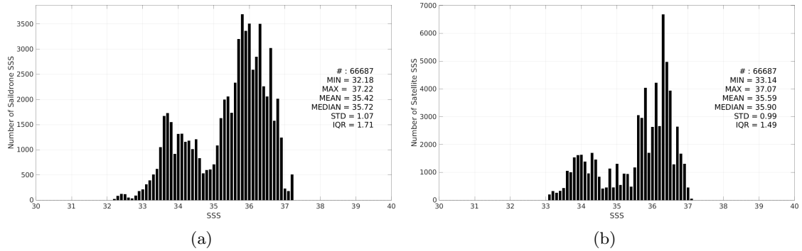
Figure 3: Histograms of SSS from Saildrone (a) and SMAP SSS L3 v5.3 - Monthly (RSS) (b) considering all match-up pairs per bins of 0.1 over the Amazon and Orinoco river plumes Pi-MEP region and for the full satellite product period.
