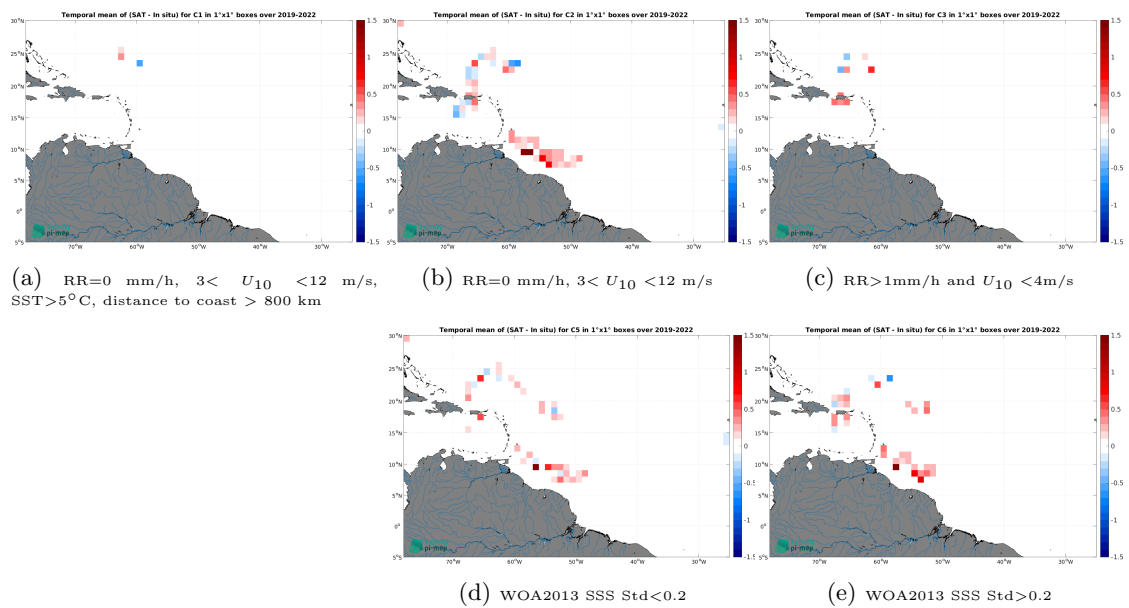
Figure 14: Temporal mean gridded over spatial boxes of size 1^\circ \times 1^\circ of \Delta SSS (SMAP SSS L3 v5.3 - Monthly (RSS) - Saldrone) for 5 different subdatasets corresponding to: RR=0 mm/h, 3 < U_{10} < 12 m/s, SST > 5°C, distance to coast > 800 km (a), RR=0 mm/h, 3 < U_{10} < 12 m/s (b), RR > 1mm/h and U_{10} < 4 m/s (c), WOA2013 SSS Std < 0.2 (d), WOA2013 SSS Std > 0.2 (e).
