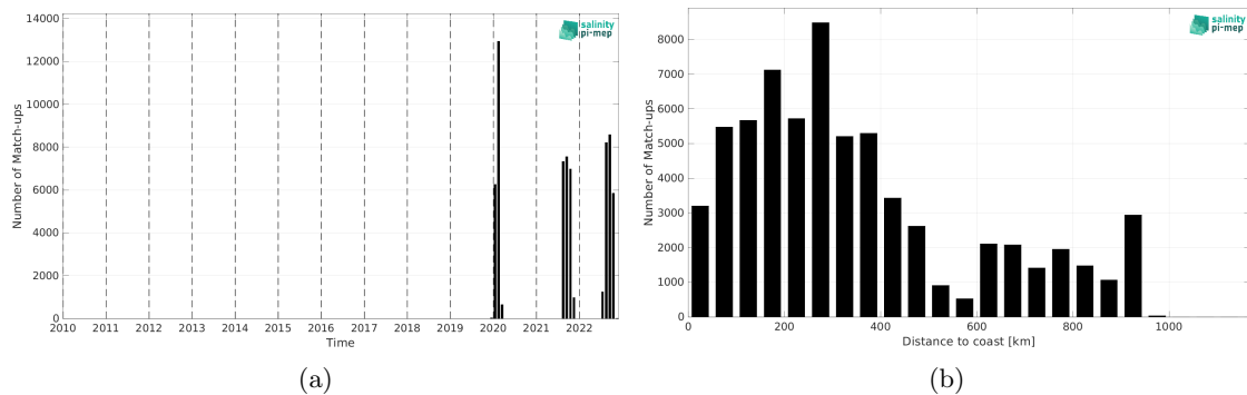
Figure 2: Number of match-ups between Saildrone and SMAP SSS L3 v5.3 - Monthly (RSS) SSS as a function of time (a) and as function of the distance to coast (b) over the Amazon and Orinoco river plumes Pi-MEP region and for the full satellite product period.
