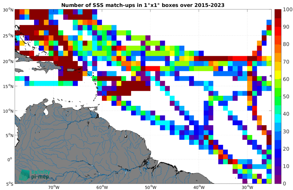
Figure 4: Number of SSS match-ups between TSG (SAMOS) SSS and the SMAP SSS L3 v5 - 8-Day running (RSS) SSS product for the Amazon and Orinoco river plumes Pi-MEP region over 1^{\circ} \times 1^{\circ} boxes and for the full satellite product period.
