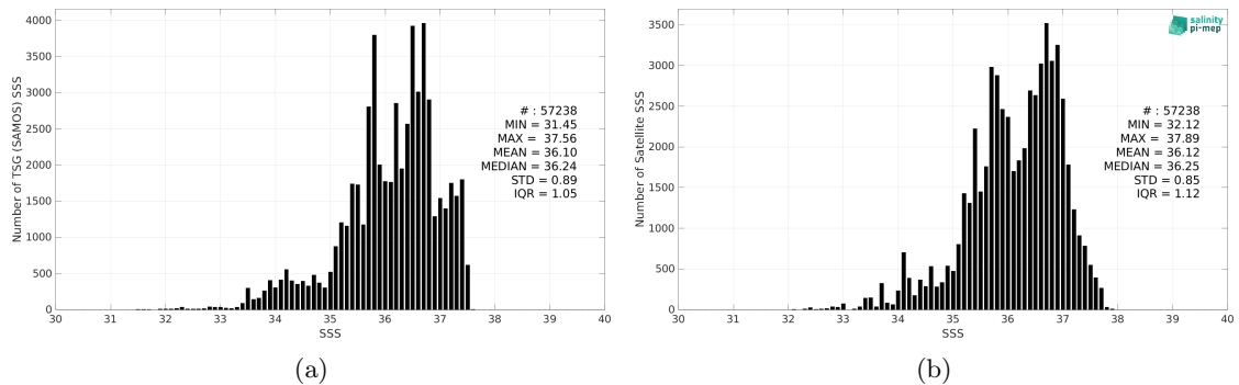
Figure 2: Histograms of SSS from TSG (SAMOS) (a) and SMAP SSS L3 v5 - 8-Day running (RSS) (b) considering all match-up pairs per bins of 0.1 over the Amazon and Orinoco river plumes Pi-MEP region and for the full satellite product period.
