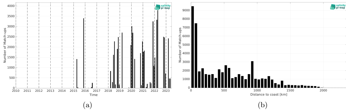
Figure 1: Number of match-ups between TSG (SAMOS) and SMAP SSS L3 v5 - 8-Day running (RSS) SSS as a function of time (a) and as function of the distance to coast (b) over the Amazon and Orinoco river plumes Pi-MEP region and for the full satellite product period.
