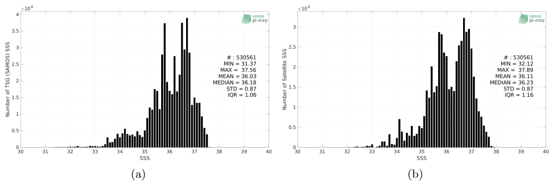
Figure 2: Histograms of SSS from TSG (SAMOS) (a) and SMAP SSS L3 v5 - 8-Day running (RSS) (b) considering all match-up pairs per bins of 0.1 over the Amazon and Orinoco river plumes Pi-MEP region and for the full satellite product period.
