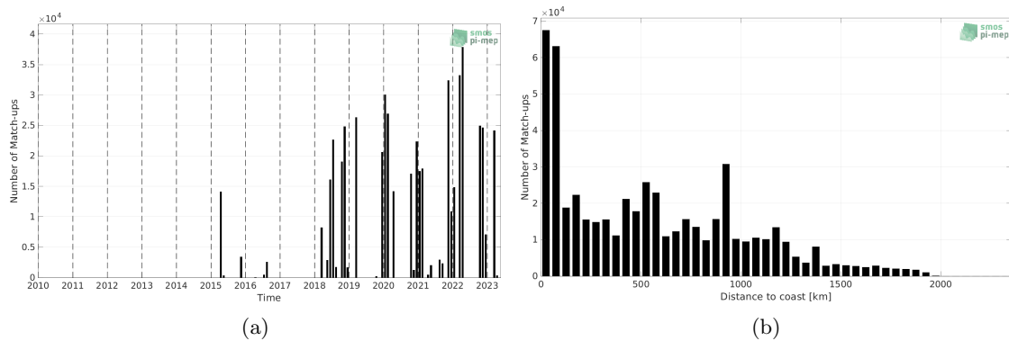
Figure 1: Number of match-ups between TSG (SAMOS) and SMAP SSS L3 v5 - 8-Day running (RSS) SSS as a function of time (a) and as function of the distance to coast (b) over the Amazon and Orinoco river plumes Pi-MEP region and for the full satellite product period.
