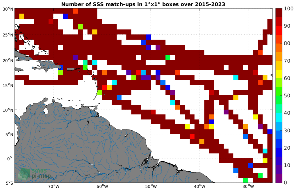
Figure 4: Number of SSS match-ups between TSG (SAMOS) SSS and the SMAP SSS L3 v5 - 8-Day running (RSS) SSS product for the Amazon and Orinoco river plumes Pi-MEP region over 1^\circ \times 1^\circ boxes and for the full satellite product period.
