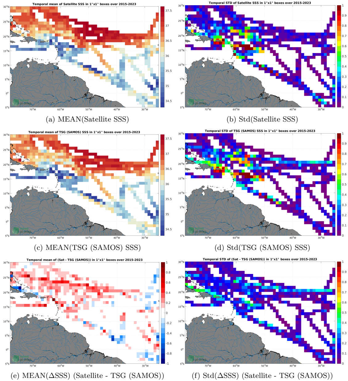
Figure 6: Temporal mean (left) and Std (right) of SSS from SMAP SSS L3 v5 - 8-Day running (RSS) (top), TSG (SAMOS) (middle), and of \Delta SSS (Satellite - TSG (SAMOS)). Only match-up pairs are used to generate these maps.
