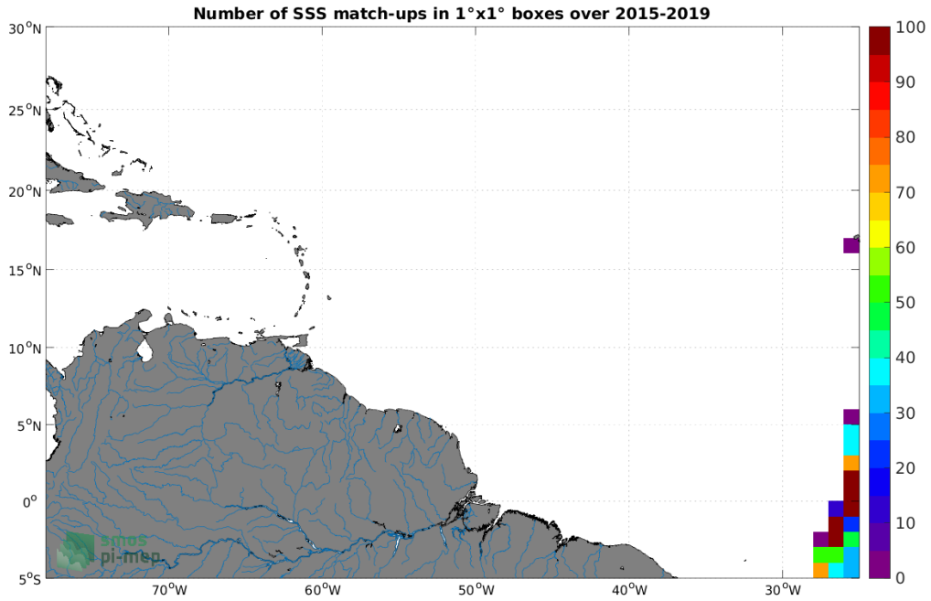
Figure 4: Number of SSS match-ups between TSG (Polarstern) SSS and the SMAP SSS L3 v5 - 8-Day running (RSS) SSS product for the Amazon and Orinoco river plumes Pi-MEP region over 1°x1° boxes and for the full satellite product period.
