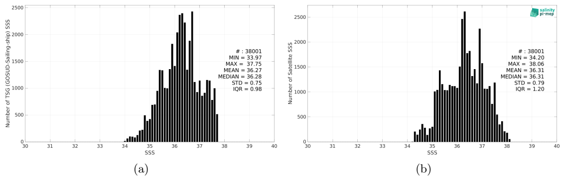
Figure 2: Histograms of SSS from TSG (GOSUD-Sailing-ship) (a) and SMAP SSS L3 v5 - 8-Day running (RSS) (b) considering all match-up pairs per bins of 0.1 over the Amazon and Orinoco river plumes Pi-MEP region and for the full satellite product period.
