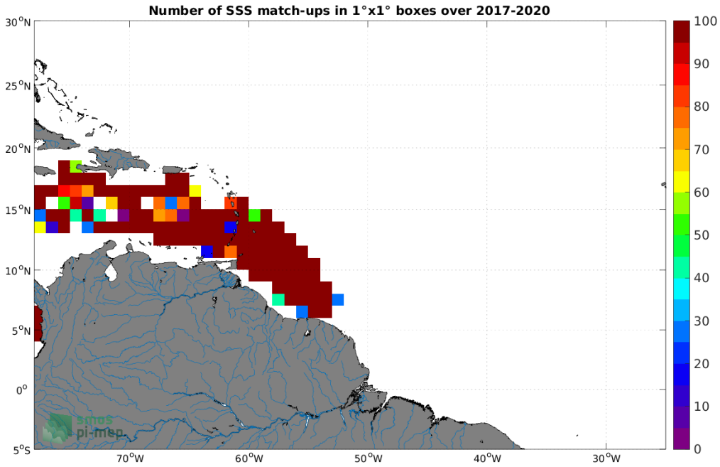
Figure 3: Number of SSS match-ups between Surface drifters SSS and the SMAP SSS L3 v5 - 8-Day running (RSS) SSS product for the Amazon and Orinoco river plumes Pi-MEP region over 1°x1° boxes and for the full satellite product period.
