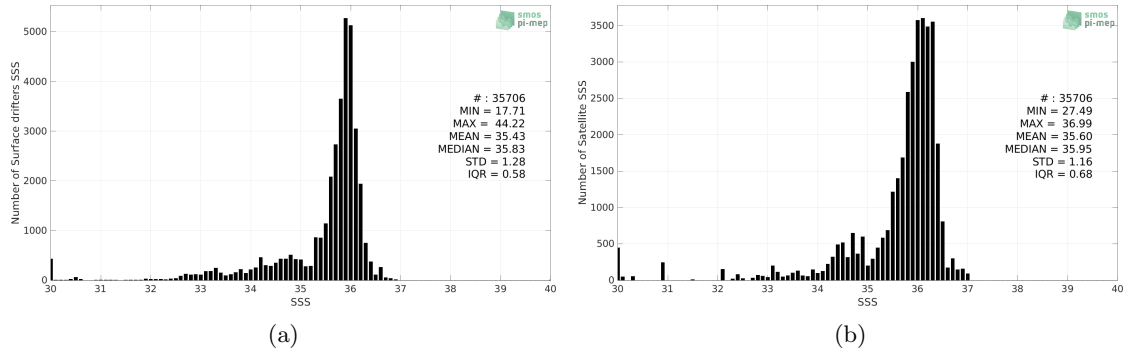
Figure 2: Histograms of SSS from Surface drifters (a) and SMAP SSS L3 v5 - 8-Day running (RSS) (b) considering all match-up pairs per bins of 0.1 over the Amazon and Orinoco river plumes Pi-MEP region and for the full satellite product period.
