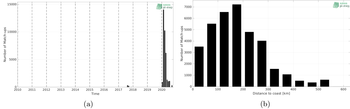
Figure 1: Number of match-ups between Surface drifters and SMAP SSS L3 v5 - 8-Day running (RSS) SSS as a function of time (a) and as function of the distance to coast (b) over the Amazon and Orinoco river plumes Pi-MEP region and for the full satellite product period.
