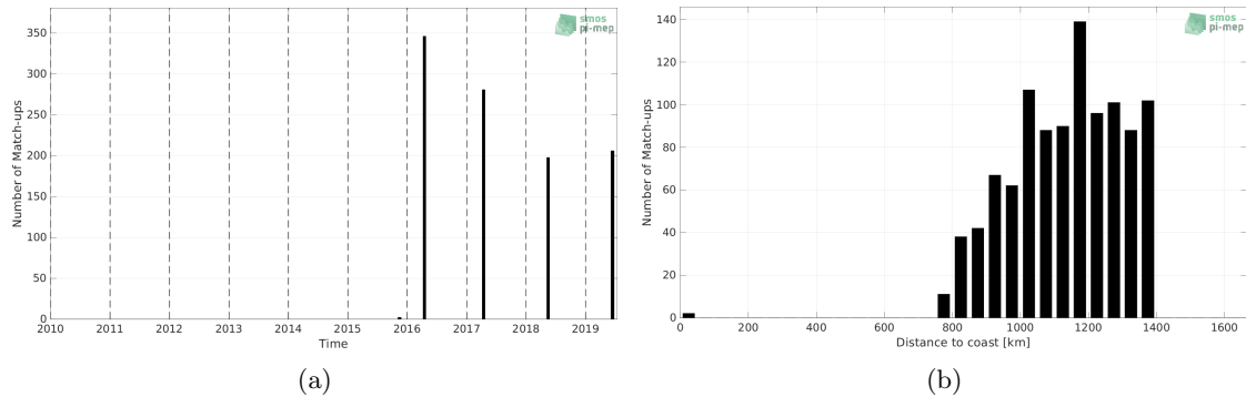
Figure 1: Number of match-ups between TSG (Polarstern) and SMAP SSS L3 v5 - Monthly (RSS) SSS as a function of time (a) and as function of the distance to coast (b) over the Amazon and Orinoco river plumes Pi-MEP region and for the full satellite product period.
