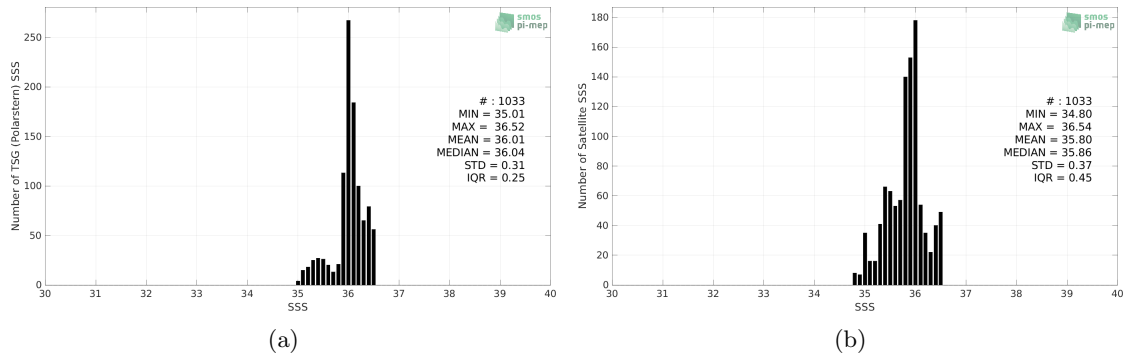
Figure 2: Histograms of SSS from TSG (Polarstern) (a) and SMAP SSS L3 v5 - Monthly (RSS) (b) considering all match-up pairs per bins of 0.1 over the Amazon and Orinoco river plumes Pi-MEP region and for the full satellite product period.
