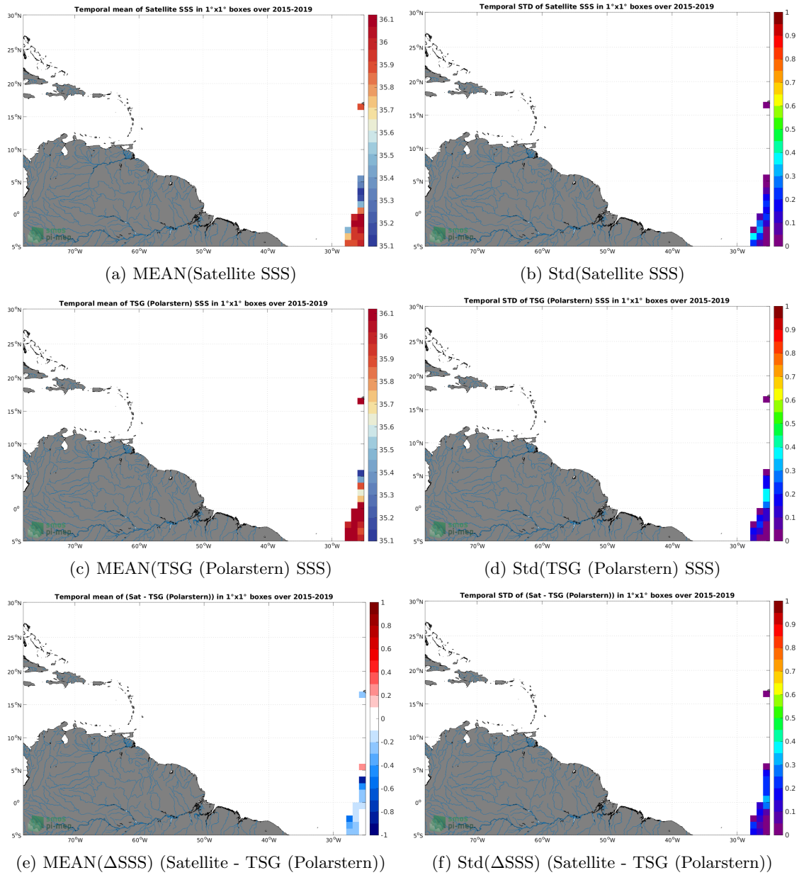
Figure 6: Temporal mean (left) and Std (right) of SSS from SMAP SSS L3 v5 - Monthly (RSS) (top), TSG (Polarstern) (middle), and of \Delta SSS (Satellite - TSG (Polarstern)). Only match-up pairs are used to generate these maps.
