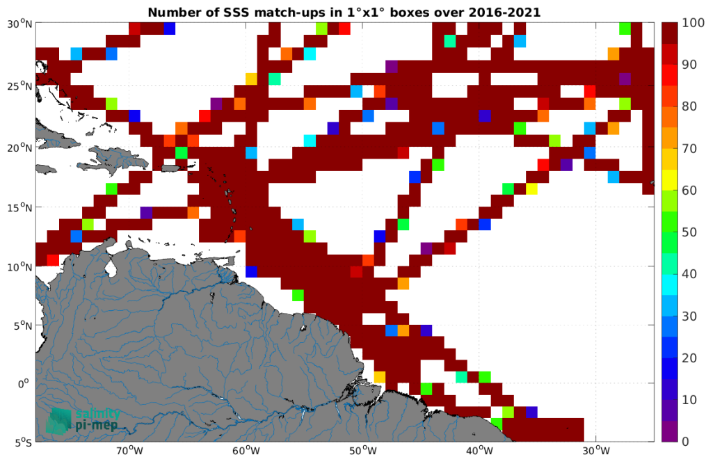
Figure 4: Number of SSS match-ups between TSG (GOSUD-Research-vessel) SSS and the SMAP SSS L3 v5 - Monthly (RSS) SSS product for the Amazon and Orinoco river plumes Pi-MEP region over 1^{\circ} \times 1^{\circ} boxes and for the full satellite product period.
