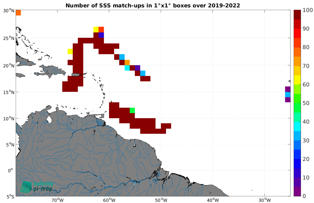
Figure 4: Number of SSS match-ups between Saildrone SSS and the SMAP SSS L3 v5 - Monthly (RSS) SSS product for the Amazon and Orinoco river plumes Pi-MEP region over 1^{\circ} \times 1^{\circ} boxes and for the full satellite product period.
