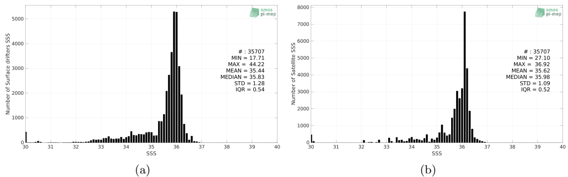
Figure 2: Histograms of SSS from Surface drifters (a) and SMAP SSS L3 v5 - Monthly (RSS) (b) considering all match-up pairs per bins of 0.1 over the Amazon and Orinoco river plumes Pi-MEP region and for the full satellite product period.
