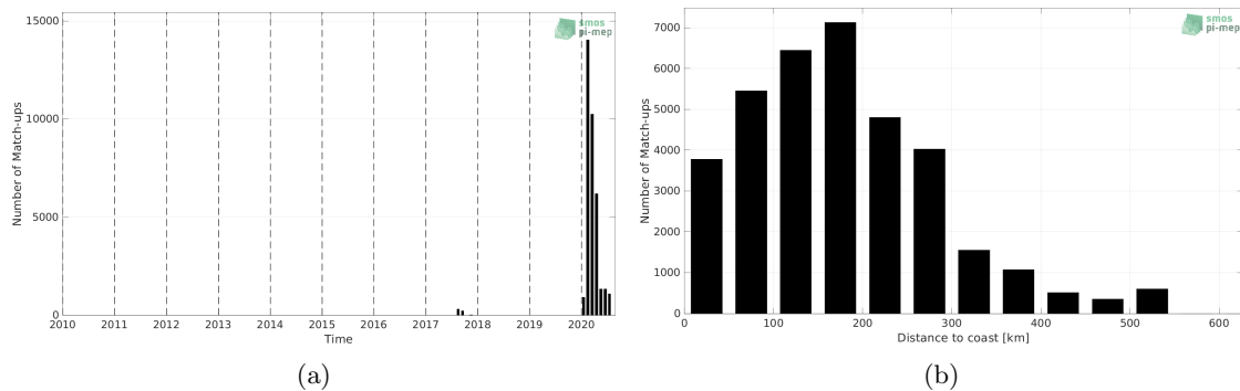
Figure 1: Number of match-ups between Surface drifters and SMAP SSS L3 v5 - Monthly (RSS) SSS as a function of time (a) and as function of the distance to coast (b) over the Amazon and Orinoco river plumes Pi-MEP region and for the full satellite product period.
