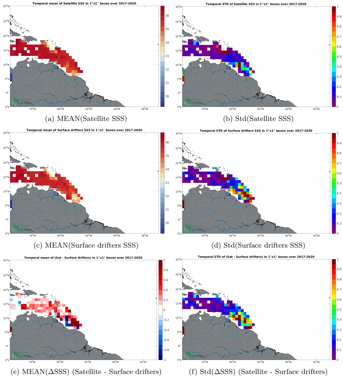
Figure 5: Temporal mean (left) and Std (right) of SSS from SMAP SSS L3 v5 - Monthly (RSS) (top), Surface drifters (middle), and of \Delta SSS (Satellite - Surface drifters). Only match-up pairs are used to generate these maps.
