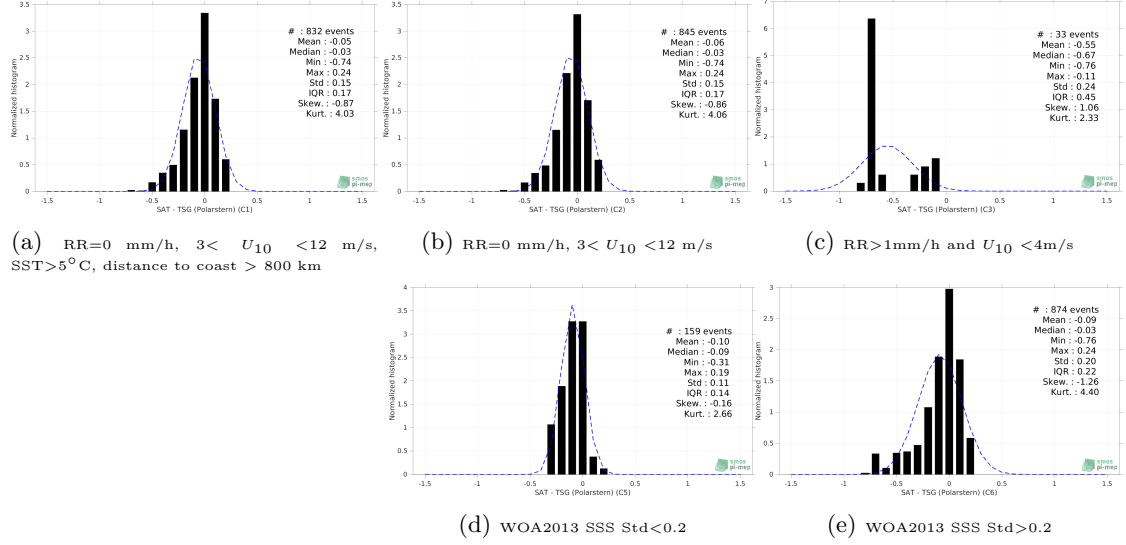
Figure 13: Normalized histogram of \Delta\text{SSS} (SMAP SSS L3 v4 - 8-Day running (RSS) - TSG (Polarstern)) for 5 different subdatasets corresponding to: RR=0 mm/h, 3 < U_{10} < 12 m/s, SST>5°C, distance to coast > 800 km (a), RR=0 mm/h, 3 < U_{10} < 12 m/s (b), RR>1mm/h and U_{10} < 4 m/s (c), WOA2013 SSS Std<0.2 (d), WOA2013 SSS Std>0.2 (e).
