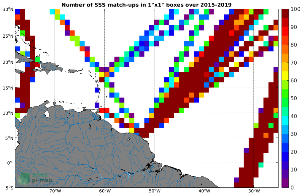
Figure 4: Number of SSS match-ups between TSG (LEGOS-DM) SSS and the SMAP SSS L3 v4 - 8-Day running (RSS) SSS product for the Amazon and Orinoco river plumes Pi-MEP region over 1°x1° boxes and for the full satellite product period.
