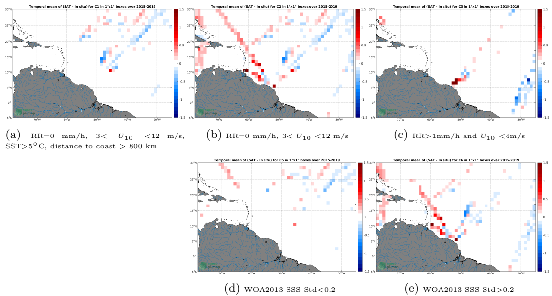
Figure 12: Temporal mean gridded over spatial boxes of size 1°x1° of \Delta SSS (SMAP SSS L3 v4 - 8-Day running (RSS) - TSG (LEGOS-DM)) for 5 different subdatasets corresponding to: RR=0 mm/h, 3 < U_{10} < 12 m/s, SST > 5°C, distance to coast > 800 km (a), RR=0 mm/h, 3 < U_{10} < 12 m/s (b), RR > 1mm/h and U_{10} < 4 m/s (c), WOA2013 SSS Std < 0.2 (d), WOA2013 SSS Std > 0.2 (e).
