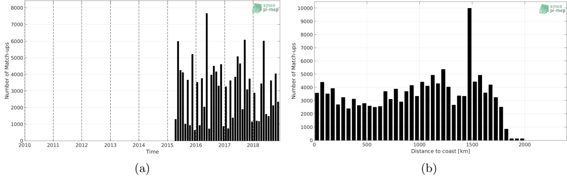
Figure 1: Number of match-ups between TSG-LEGOS-DM and SMAP-L3-RSS-V4-8DAY-RUNNING SSS as a function of time (a) and as function of the distance to coast (b) over the Amazon and Orinoco river plumes Pi-MEP region and for the full satellite product period.
