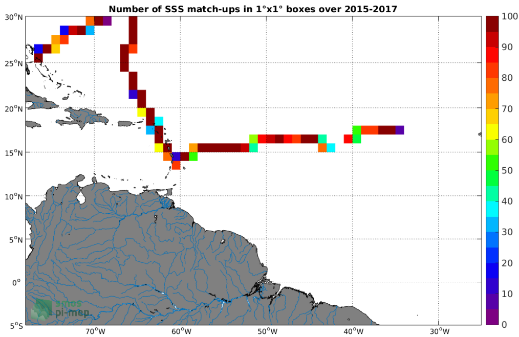
Figure 4: Number of SSS match-ups between TSG-GOSUD-Sailing-ship SSS and the SMAP-L3-RSS-V4-8DAY-RUNNING SSS product for the Amazon and Orinoco river plumes Pi-MEP region over 1°x1° boxes and for the full satellite product period.
