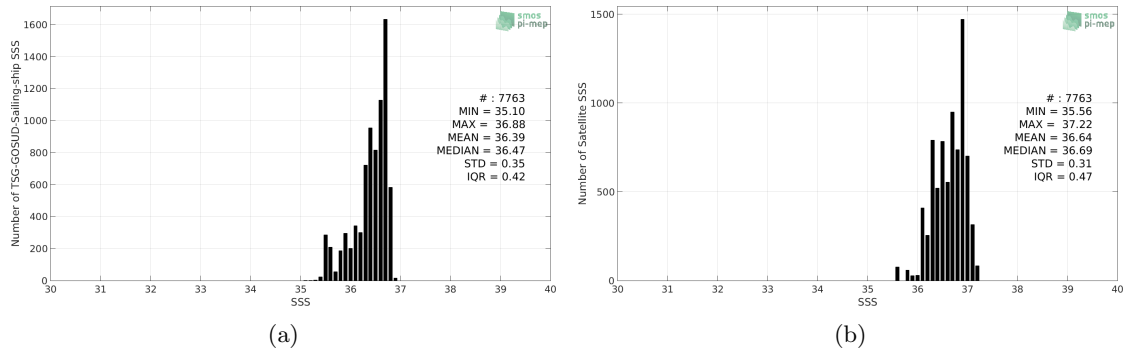
Figure 2: Histograms of SSS from TSG-GOSUD-Sailing-ship (a) and SMAP-L3-RSS-V4-8DAY-RUNNING (b) considering all match-up pairs per bins of 0.1 over the Amazon and Orinoco river plumes Pi-MEP region and for the full satellite product period.
