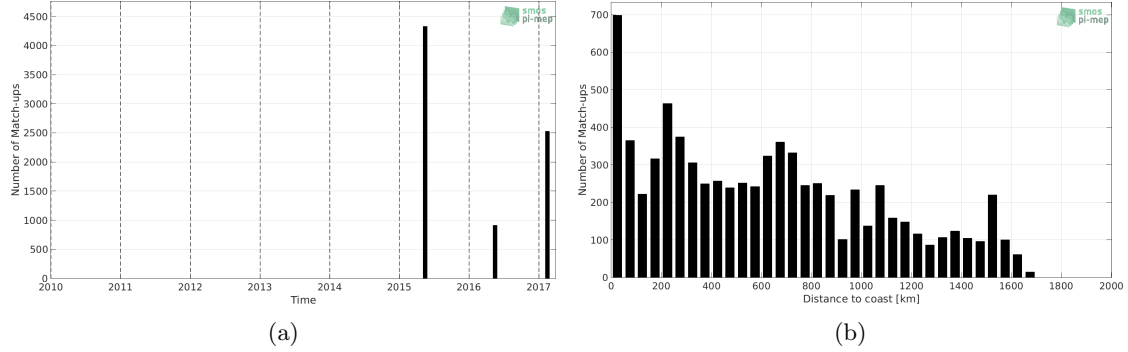
Figure 1: Number of match-ups between TSG-GOSUD-Sailing-ship and SMAP-L3-RSS-V4-8DAY-RUNNING SSS as a function of time (a) and as function of the distance to coast (b) over the Amazon and Orinoco river plumes Pi-MEP region and for the full satellite product period.
