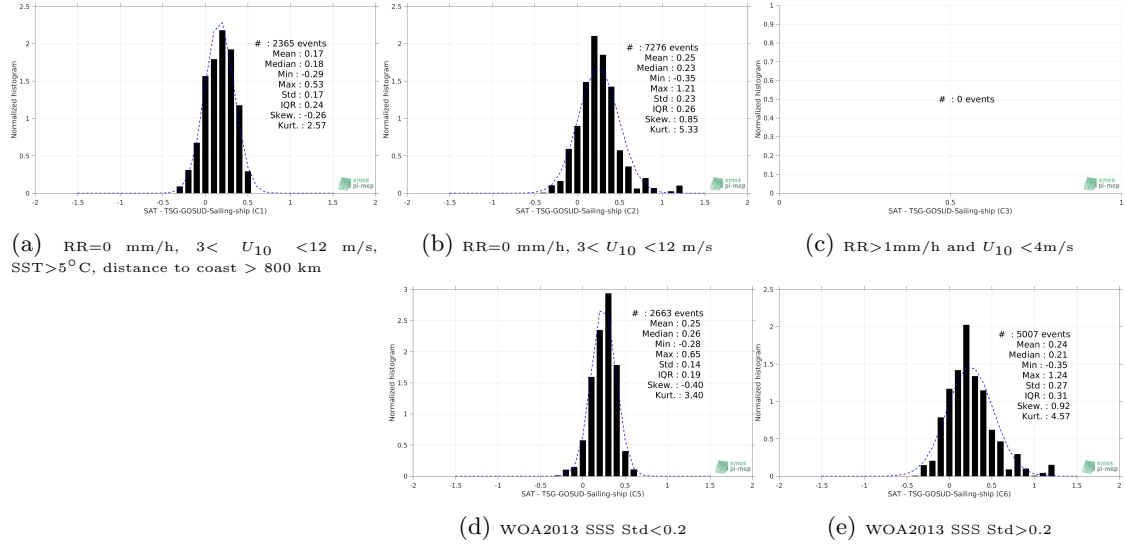
Figure 13: Normalized histogram of \Delta\text{SSS} (SMAP-L3-RSS-V4-8DAY-RUNNING - TSG-GOSUD-Sailing-ship) for 5 different subdatasets corresponding to: RR=0 mm/h, 3 < U_{10} < 12 m/s, SST > 5^\circ\text{C} , distance to coast > 800 km (a), RR=0 mm/h, 3 < U_{10} < 12 m/s (b), RR > 1 mm/h and U_{10} < 4 m/s (c), WOA2013 SSS Std < 0.2 (d), WOA2013 SSS Std > 0.2 (e).
