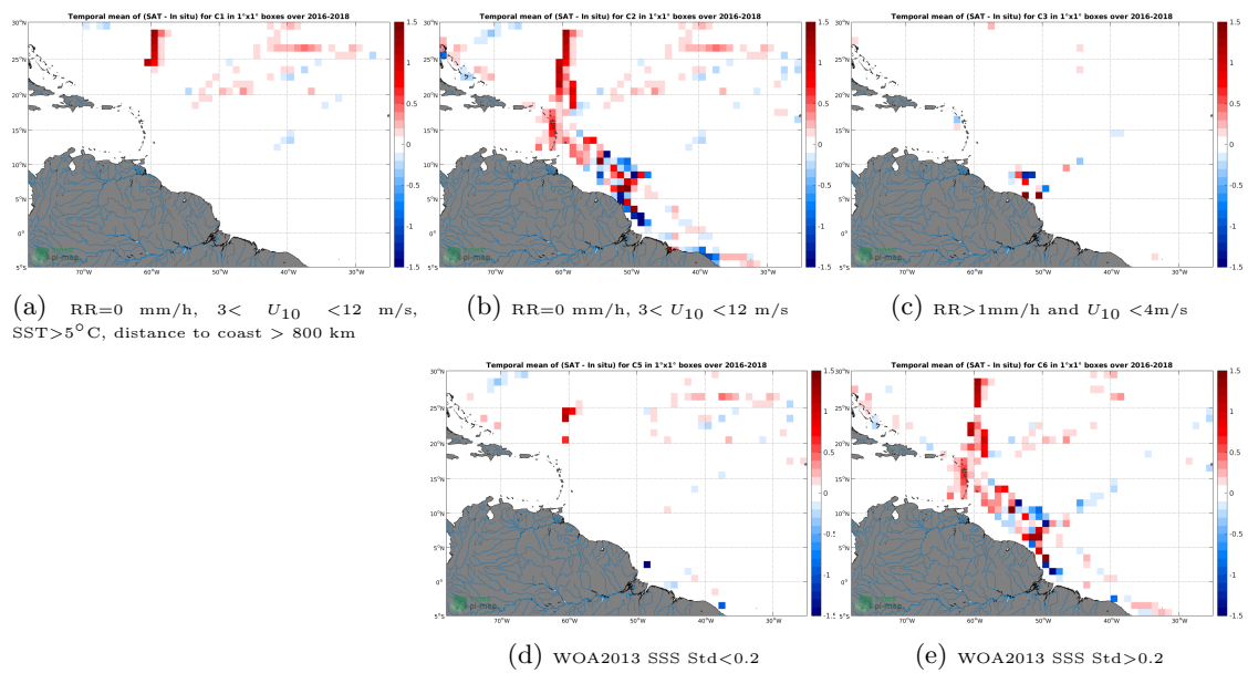
Figure 12: Temporal mean gridded over spatial boxes of size 1^\circ \times 1^\circ of \Delta\text{SSS} (SMAP-L3-RSS-V4-8DAY-RUNNING - TSG-GOSUD-Research-vessel) for 5 different subdatasets corresponding to:RR=0 mm/h, 3 < U_{10} < 12 m/s, SST>5°C, distance to coast > 800 km (a), RR=0 mm/h, 3 < U_{10} < 12 m/s (b), RR>1mm/h and U_{10} < 4 m/s (c), WOA2013 SSS Std<0.2 (d), WOA2013 SSS Std>0.2 (e).
