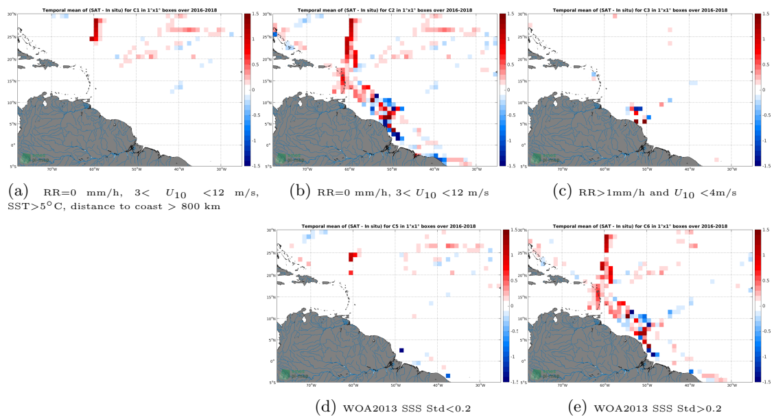
Figure 12: Temporal mean gridded over spatial boxes of size 1^\circ \times 1^\circ of \Delta SSS (SMAP-L3-RSS-V4-8DAY-RUNNING - TSG-GOSUD-Research-vessel) for 5 different subdatasets corresponding to:RR=0 mm/h, 3 < U_{10} < 12 m/s, SST>5°C, distance to coast > 800 km (a), RR=0 mm/h, 3 < U_{10} < 12 m/s (b), RR>1mm/h and U_{10} < 4 m/s (c), WOA2013 SSS Std<0.2 (d), WOA2013 SSS Std>0.2 (e).
