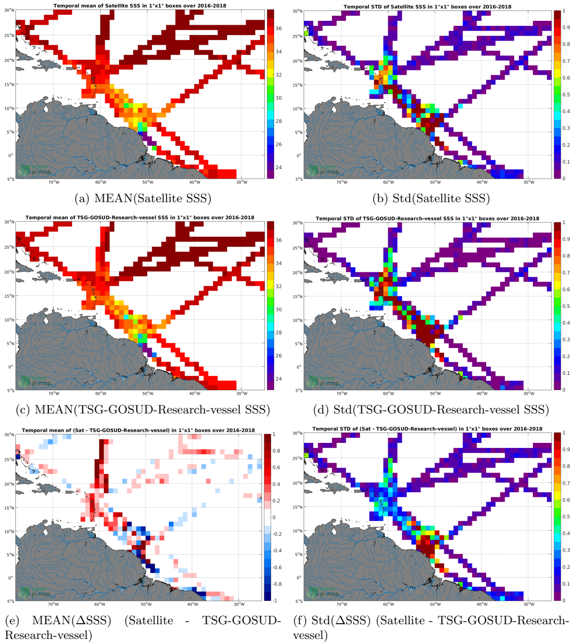
Figure 6: Temporal mean (left) and Std (right) of SSS from SMAP-L3-RSS-V4-8DAY-RUNNING (top), TSG-GOSUD-Research-vessel (middle), and of \Delta SSS (Satellite - TSG-GOSUD-Research-vessel). Only match-up pairs are used to generate these maps.
