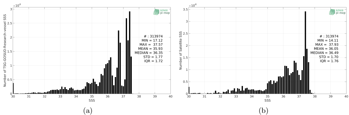
Figure 2: Histograms of SSS from TSG-GOSUD-Research-vessel (a) and SMAP-L3-RSS-V4-8DAY-RUNNING (b) considering all match-up pairs per bins of 0.1 over the Amazon and Orinoco river plumes Pi-MEP region and for the full satellite product period.
