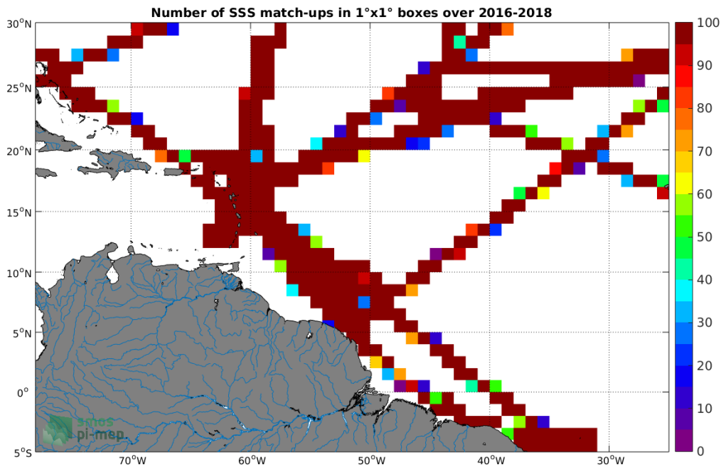
Figure 4: Number of SSS match-ups between TSG-GOSUD-Research-vessel SSS and the SMAP-L3-RSS-V4-8DAY-RUNNING SSS product for the Amazon and Orinoco river plumes Pi-MEP region over 1°x1° boxes and for the full satellite product period.
