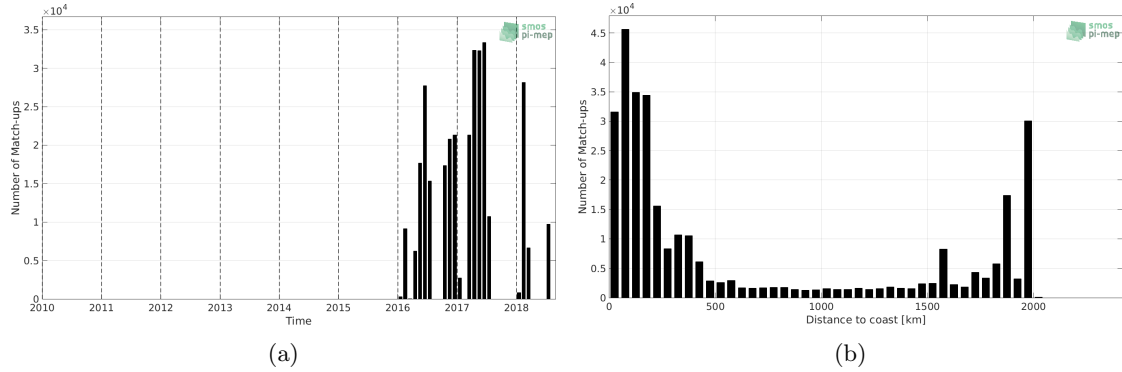
Figure 1: Number of match-ups between TSG-GOSUD-Research-vessel and SMAP-L3-RSS-V4-8DAY-RUNNING SSS as a function of time (a) and as function of the distance to coast (b) over the Amazon and Orinoco river plumes Pi-MEP region and for the full satellite product period.
