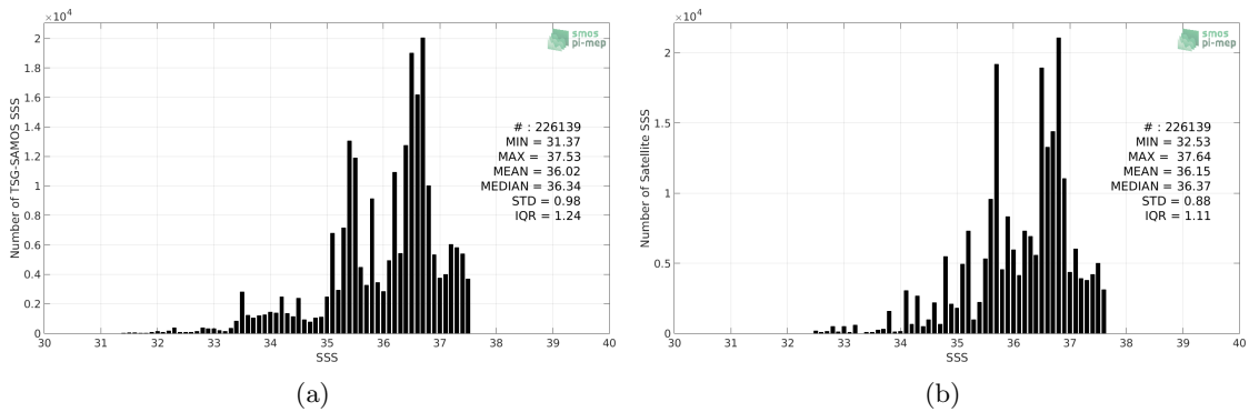
Figure 2: Histograms of SSS from TSG-SAMOS (a) and SMAP-L3-RSS-V4-MONTHLY (b) considering all match-up pairs per bins of 0.1 over the Amazon and Orinoco river plumes Pi-MEP region and for the full satellite product period.
