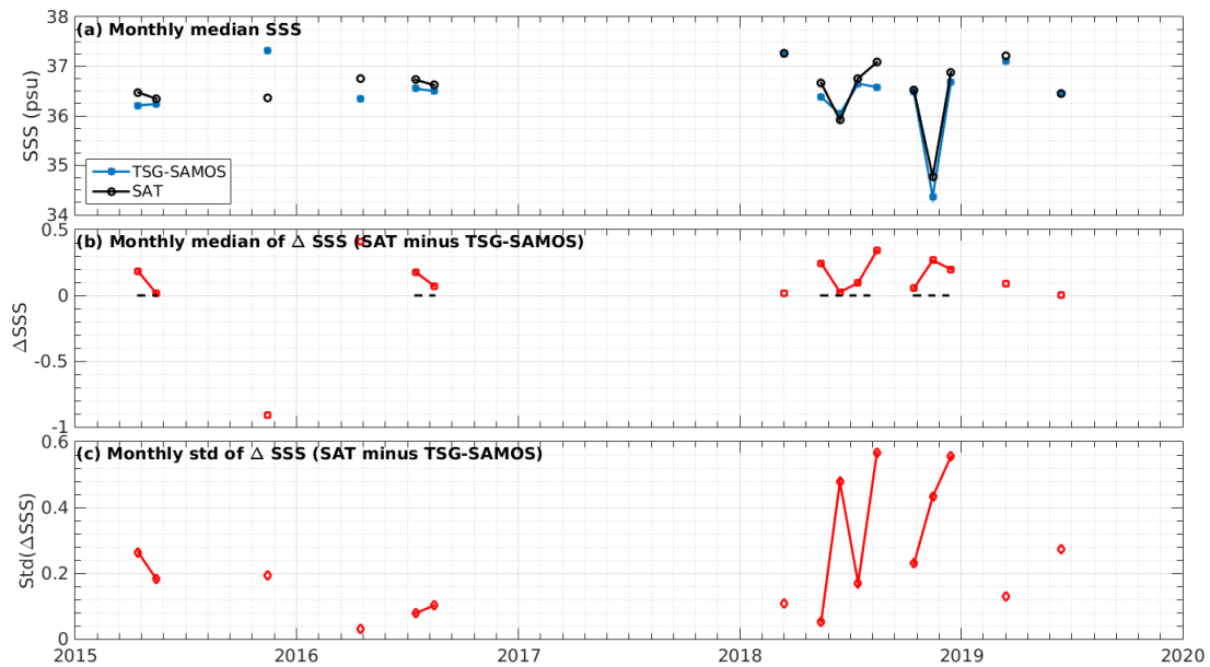
Figure 7: Time series of the monthly median SSS (top), median of \Delta\text{SSS} (Satellite - TSG-SAMOS) and Std of \Delta\text{SSS} (Satellite - TSG-SAMOS) over the Amazon and Orinoco river plumes Pi-MEP region considering all match-ups collected by the Pi-MEP.
