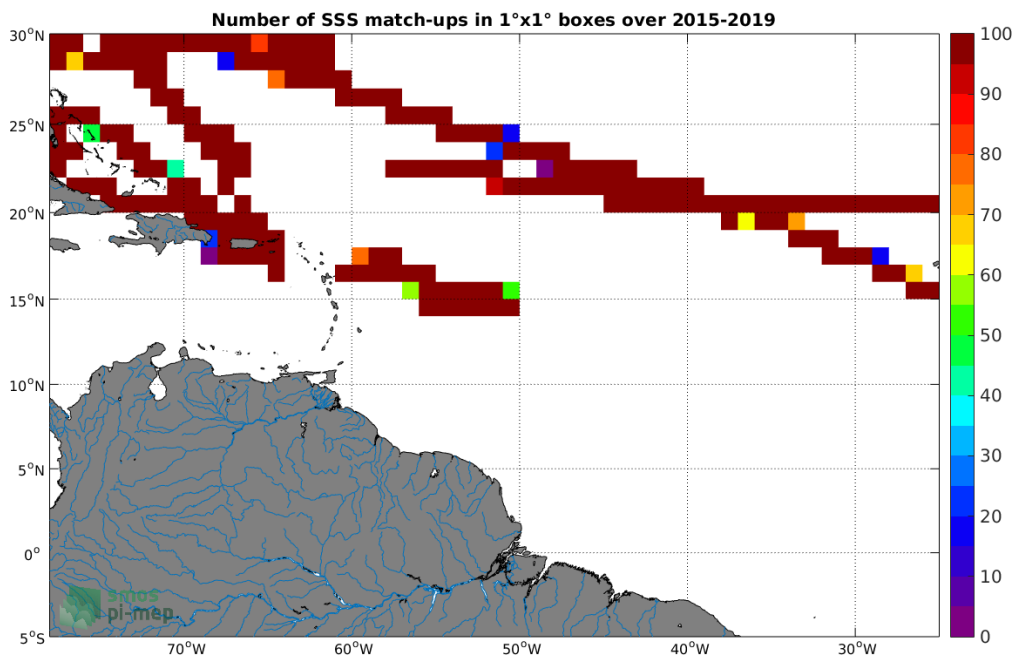
Figure 4: Number of SSS match-ups between TSG-SAMOS SSS and the SMAP-L3-RSS-V4-MONTHLY SSS product for the Amazon and Orinoco river plumes Pi-MEP region over 1^\circ \times 1^\circ boxes and for the full satellite product period.
