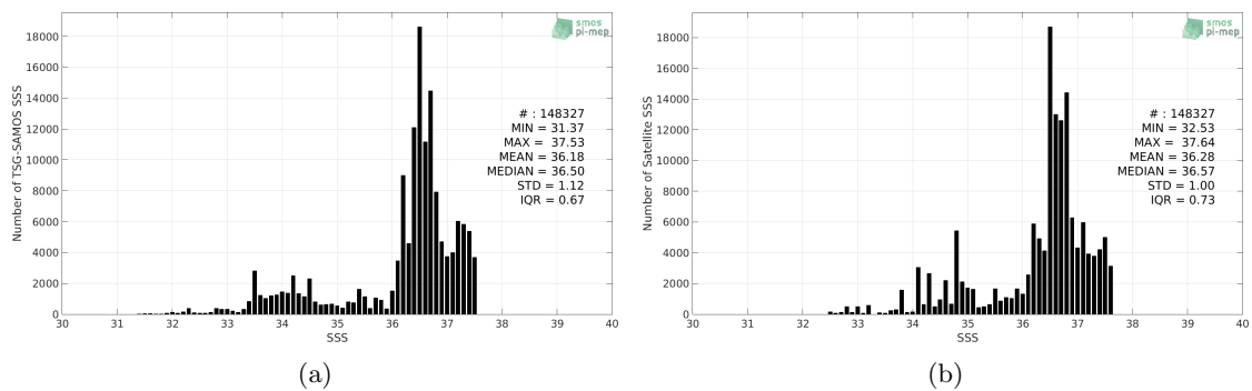
Figure 2: Histograms of SSS from TSG-SAMOS (a) and SMAP-L3-RSS-V4-MONTHLY (b) considering all match-up pairs per bins of 0.1 over the Amazon and Orinoco river plumes Pi-MEP region and for the full satellite product period.
