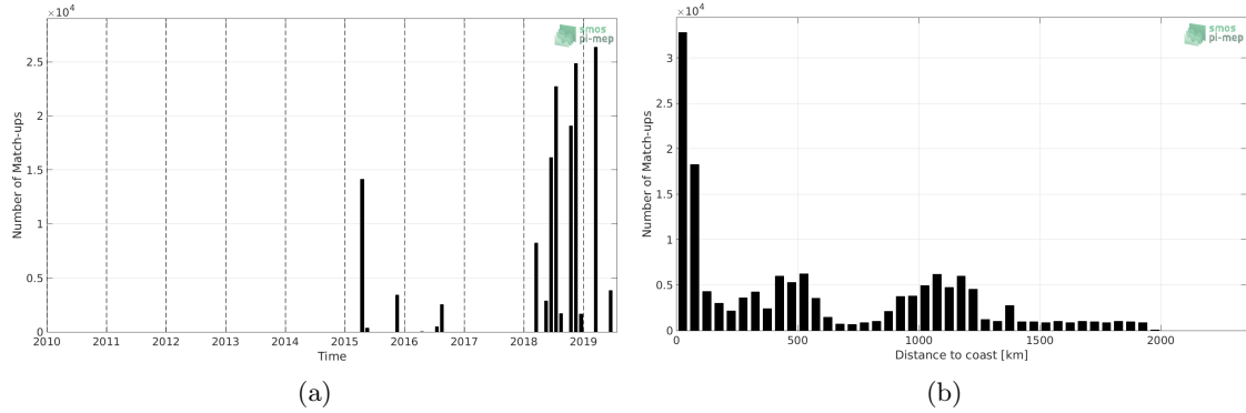
Figure 1: Number of match-ups between TSG-SAMOS and SMAP-L3-RSS-V4-MONTHLY SSS as a function of time (a) and as function of the distance to coast (b) over the Amazon and Orinoco river plumes Pi-MEP region and for the full satellite product period.
