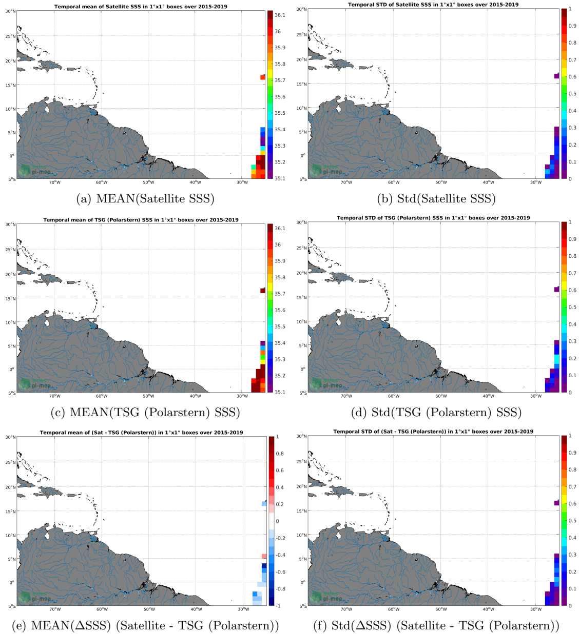
Figure 6: Temporal mean (left) and Std (right) of SSS from SMAP SSS L3 v4 - Monthly (RSS) (top), TSG (Polarstern) (middle), and of \Delta SSS (Satellite - TSG (Polarstern)). Only match-up pairs are used to generate these maps.
