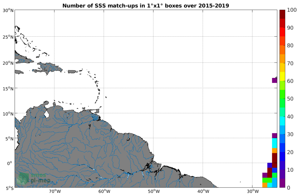
Figure 4: Number of SSS match-ups between TSG (Polarstern) SSS and the SMAP SSS L3 v4 - Monthly (RSS) SSS product for the Amazon and Orinoco river plumes Pi-MEP region over 1°x1° boxes and for the full satellite product period.
