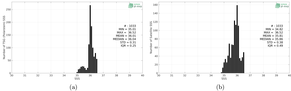
Figure 2: Histograms of SSS from TSG (Polarstern) (a) and SMAP SSS L3 v4 - Monthly (RSS) (b) considering all match-up pairs per bins of 0.1 over the Amazon and Orinoco river plumes Pi-MEP region and for the full satellite product period.
