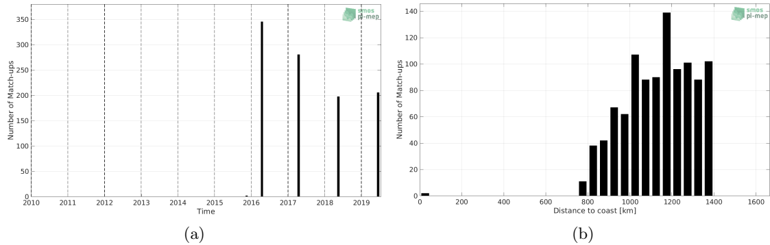
Figure 1: Number of match-ups between TSG (Polarstern) and SMAP SSS L3 v4 - Monthly (RSS) SSS as a function of time (a) and as function of the distance to coast (b) over the Amazon and Orinoco river plumes Pi-MEP region and for the full satellite product period.
