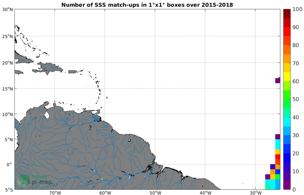
Figure 4: Number of SSS match-ups between TSG (Polarstern) SSS and the SMAP SSS L3 v4 - Monthly (RSS) SSS product for the Amazon and Orinoco river plumes Pi-MEP region over 1^\circ \times 1^\circ boxes and for the full satellite product period.
