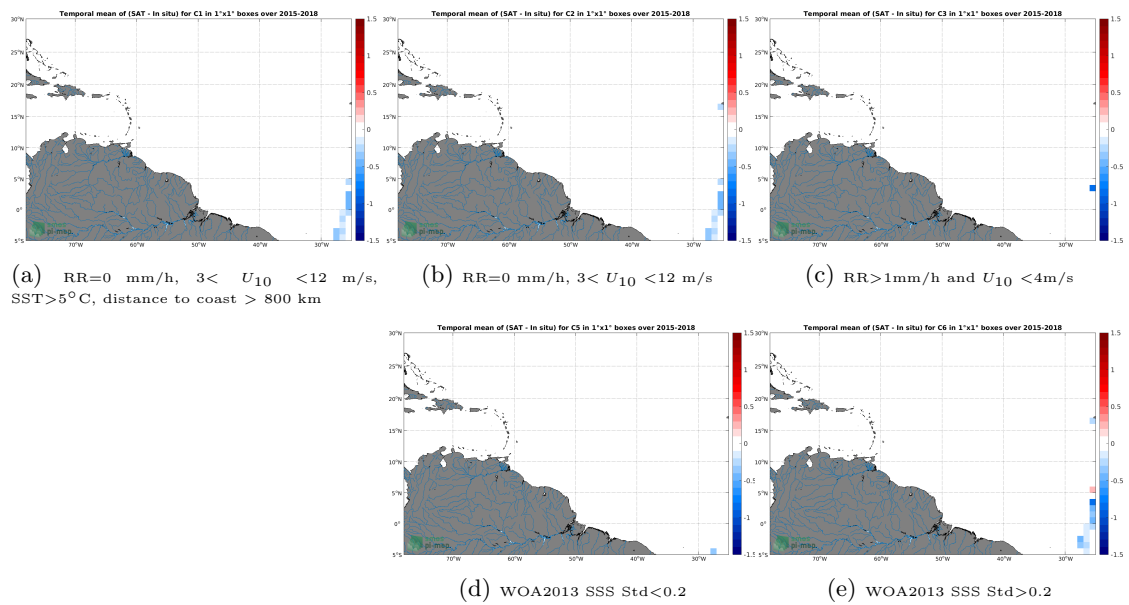
Figure 12: Temporal mean gridded over spatial boxes of size 1°x1° of \Delta SSS (SMAP SSS L3 v4 - Monthly (RSS) - TSG (Polarstern)) for 5 different subdatasets corresponding to:RR=0 mm/h, 3 < U_{10} < 12 m/s, SST>5°C, distance to coast > 800 km (a), RR=0 mm/h, 3 < U_{10} < 12 m/s (b), RR>1mm/h and U_{10} < 4 m/s (c), WOA2013 SSS Std<0.2 (d), WOA2013 SSS Std>0.2 (e).
