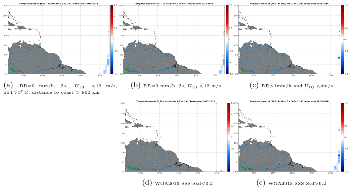
Figure 12: Temporal mean gridded over spatial boxes of size 1^\circ \times 1^\circ of \Delta SSS (SMAP-L3-RSS-V4-MONTHLY - TSG-POLARSTERN) for 5 different subdatasets corresponding to:RR=0 mm/h, 3 < U_{10} < 12 m/s, SST >5^\circ\text{C} , distance to coast > 800 km (a), RR=0 mm/h, 3 < U_{10} < 12 m/s (b), RR >1 mm/h and U_{10} < 4 m/s (c), WOA2013 SSS Std <0.2 (d), WOA2013 SSS Std >0.2 (e).
