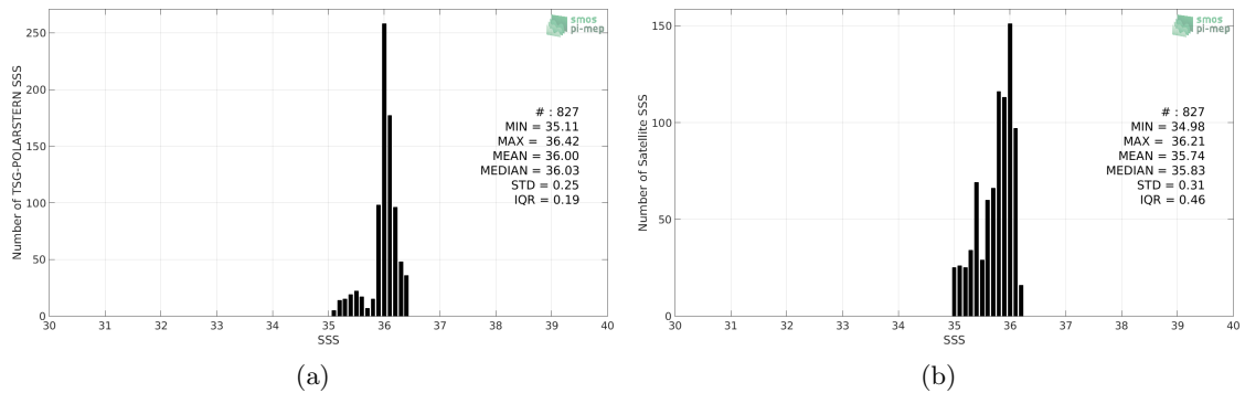
Figure 2: Histograms of SSS from TSG-POLARSTERN (a) and SMAP-L3-RSS-V4-MONTHLY (b) considering all match-up pairs per bins of 0.1 over the Amazon and Orinoco river plumes Pi-MEP region and for the full satellite product period.
