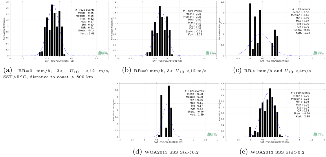
Figure 13: Normalized histogram of \Delta SSS (SMAP-L3-RSS-V4-MONTHLY - TSG-POLARSTERN) for 5 different subdatasets corresponding to: RR=0 mm/h, 3 < U_{10} < 12 m/s, SST > 5°C, distance to coast > 800 km (a), RR=0 mm/h, 3 < U_{10} < 12 m/s (b), RR > 1mm/h and U_{10} < 4 m/s (c), WOA2013 SSS Std < 0.2 (d), WOA2013 SSS Std > 0.2 (e).
