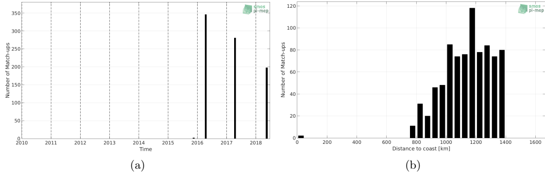
Figure 1: Number of match-ups between TSG-POLARSTERN and SMAP-L3-RSS-V4-MONTHLY SSS as a function of time (a) and as function of the distance to coast (b) over the Amazon and Orinoco river plumes Pi-MEP region and for the full satellite product period.
