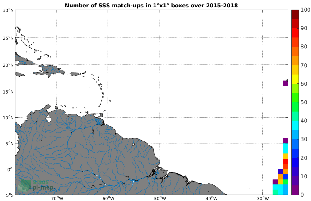
Figure 4: Number of SSS match-ups between TSG-POLARSTERN SSS and the SMAP-L3-RSS-V4-MONTHLY SSS product for the Amazon and Orinoco river plumes Pi-MEP region over 1^\circ \times 1^\circ boxes and for the full satellite product period.
