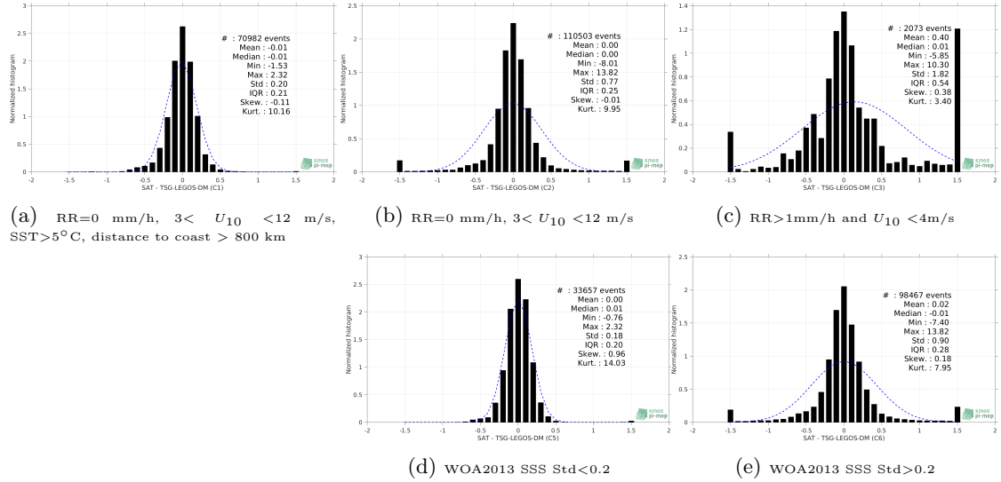
Figure 13: Normalized histogram of \Delta\text{SSS} (SMAP-L3-RSS-V4-MONTHLY - TSG-LEGOS-DM) for 5 different subdatasets corresponding to: RR=0 mm/h, 3 < U_{10} < 12 m/s, SST > 5^\circ\text{C} , distance to coast > 800 km (a), RR=0 mm/h, 3 < U_{10} < 12 m/s (b), RR > 1 mm/h and U_{10} < 4 m/s (c), WOA2013 SSS Std < 0.2 (d), WOA2013 SSS Std > 0.2 (e).
