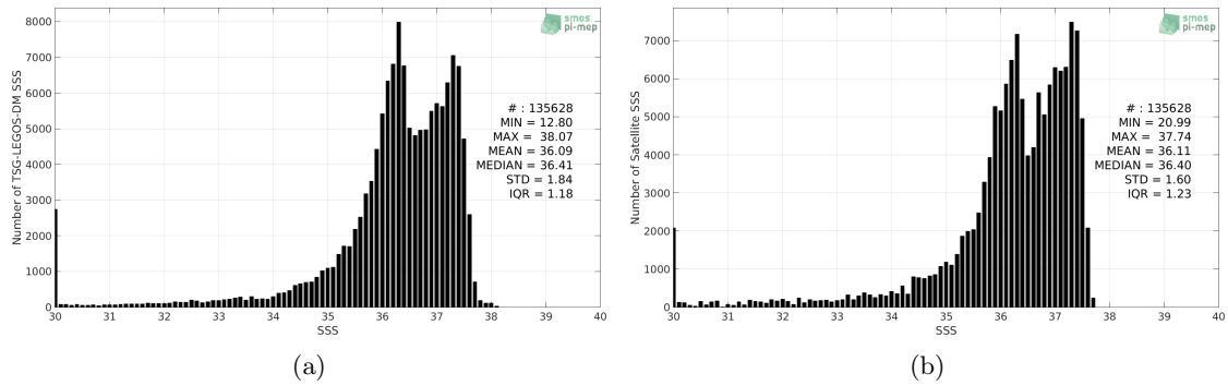
Figure 2: Histograms of SSS from TSG-LEGOS-DM (a) and SMAP-L3-RSS-V4-MONTHLY (b) considering all match-up pairs per bins of 0.1 over the Amazon and Orinoco river plumes Pi-MEP region and for the full satellite product period.
