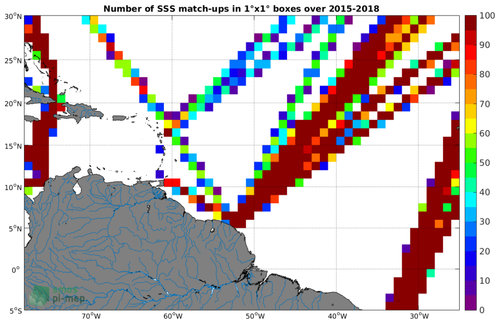
Figure 4: Number of SSS match-ups between TSG-LEGOS-DM SSS and the SMAP-L3-RSS-V4-MONTHLY SSS product for the Amazon and Orinoco river plumes Pi-MEP region over 1^\circ \times 1^\circ boxes and for the full satellite product period.
