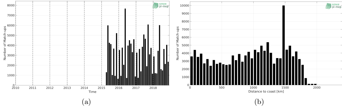
Figure 1: Number of match-ups between TSG-LEGOS-DM and SMAP-L3-RSS-V4-MONTHLY SSS as a function of time (a) and as function of the distance to coast (b) over the Amazon and Orinoco river plumes Pi-MEP region and for the full satellite product period.
