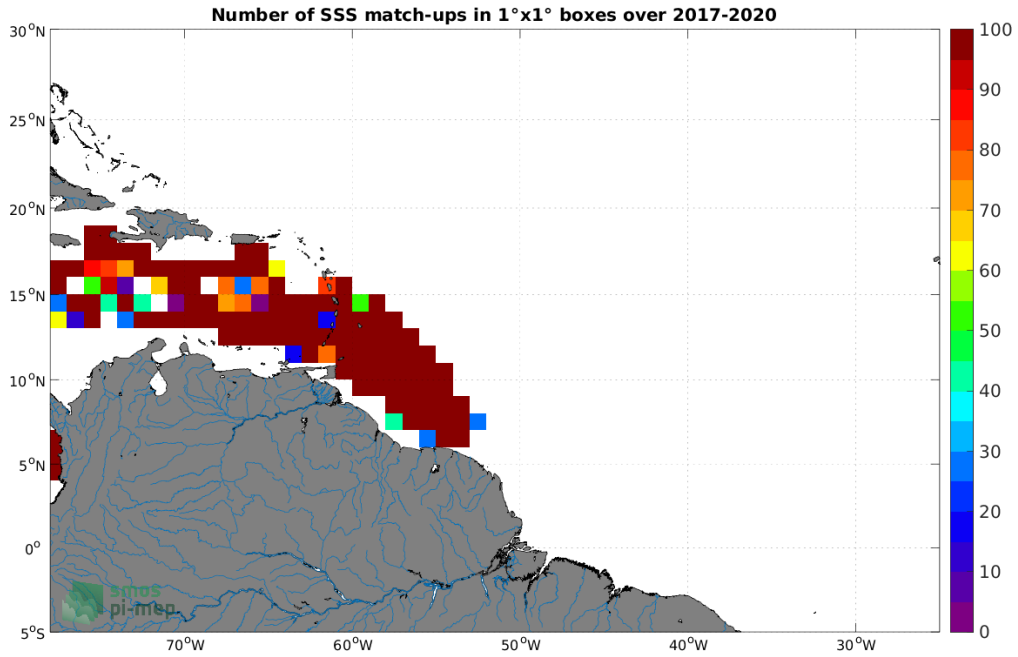
Figure 3: Number of SSS match-ups between Surface drifters SSS and the SMAP SSS L3 v4 - Monthly (RSS) SSS product for the Amazon and Orinoco river plumes Pi-MEP region over 1°x1° boxes and for the full satellite product period.
