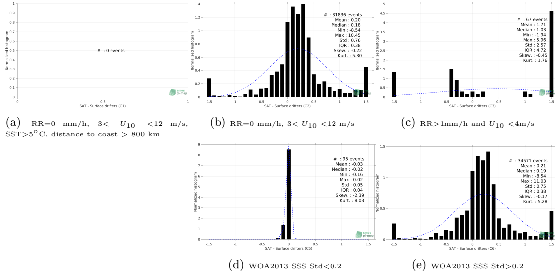
Figure 12: Normalized histogram of \Delta\text{SSS} (SMAP SSS L3 v4 - Monthly (RSS) - Surface drifters) for 5 different subdatasets corresponding to: RR=0 mm/h, 3 < U_{10} < 12 m/s, SST > 5^\circ\text{C} , distance to coast > 800 km (a), RR=0 mm/h, 3 < U_{10} < 12 m/s (b), RR > 1\text{mm/h} and U_{10} < 4\text{m/s} (c), WOA2013 SSS \text{Std} < 0.2 (d), WOA2013 SSS \text{Std} > 0.2 (e).
