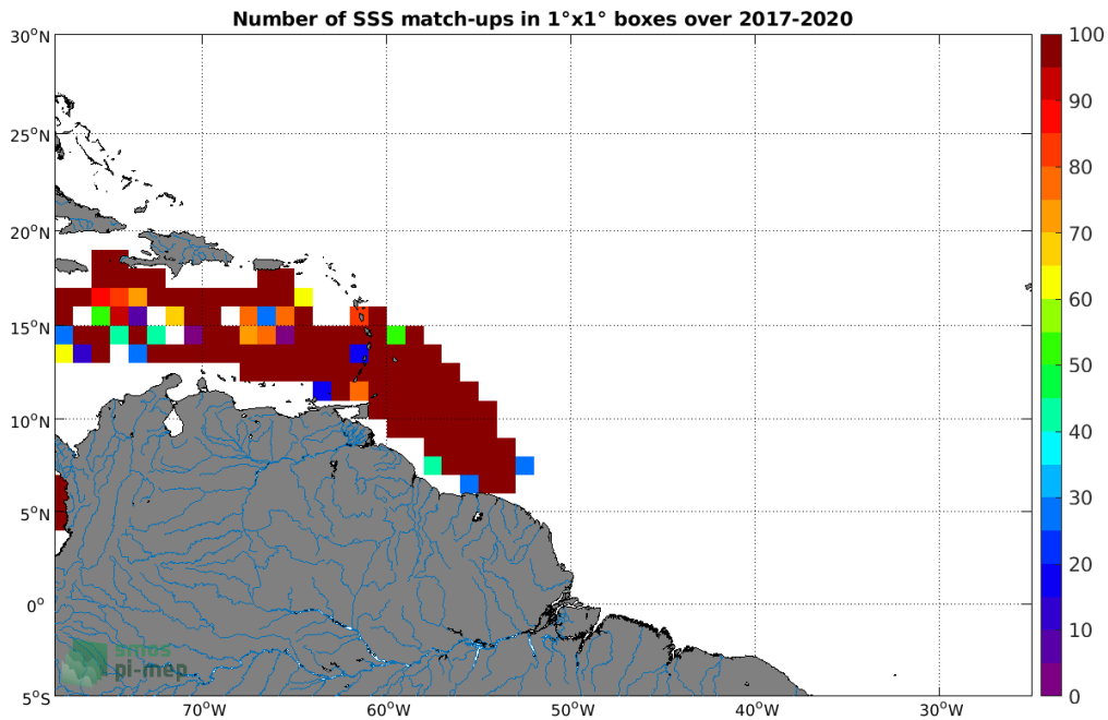
Figure 3: Number of SSS match-ups between Surface drifters SSS and the SMAP SSS L3 v4 - Monthly (RSS) SSS product for the Amazon and Orinoco river plumes Pi-MEP region over 1^\circ \times 1^\circ boxes and for the full satellite product period.
