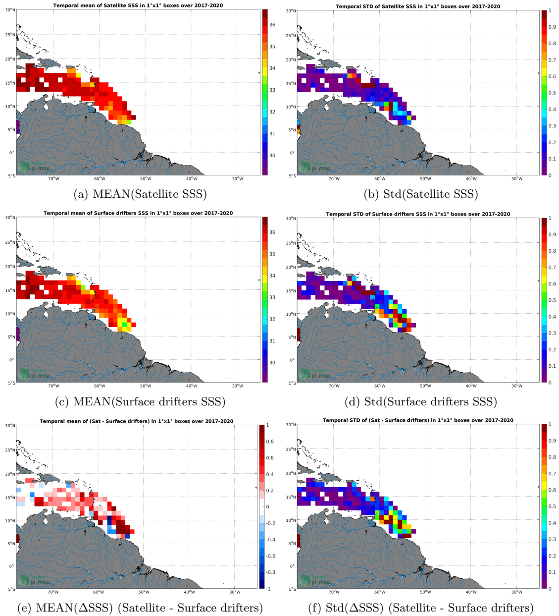
Figure 5: Temporal mean (left) and Std (right) of SSS from SMAP SSS L3 v4 - Monthly (RSS) (top), Surface drifters (middle), and of \Delta SSS (Satellite - Surface drifters). Only match-up pairs are used to generate these maps.
