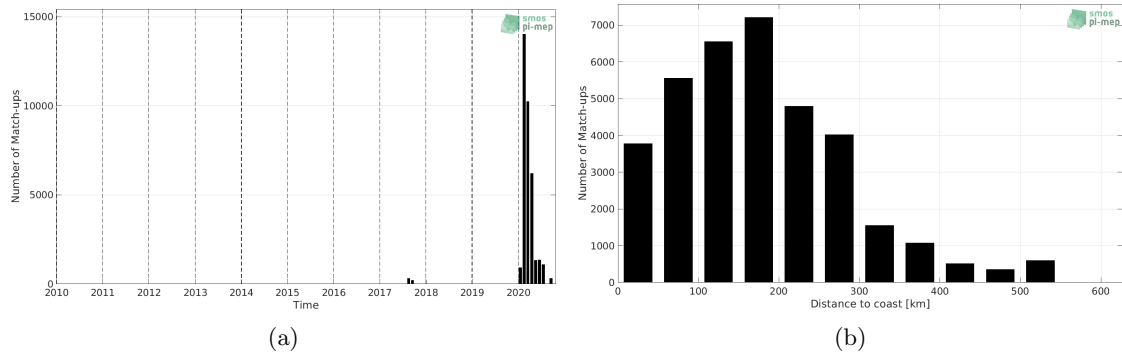
Figure 1: Number of match-ups between Surface drifters and SMAP SSS L3 v4 - Monthly (RSS) SSS as a function of time (a) and as function of the distance to coast (b) over the Amazon and Orinoco river plumes Pi-MEP region and for the full satellite product period.
