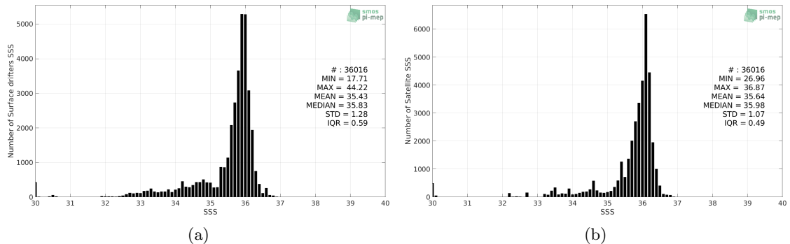
Figure 2: Histograms of SSS from Surface drifters (a) and SMAP SSS L3 v4 - Monthly (RSS) (b) considering all match-up pairs per bins of 0.1 over the Amazon and Orinoco river plumes Pi-MEP region and for the full satellite product period.
