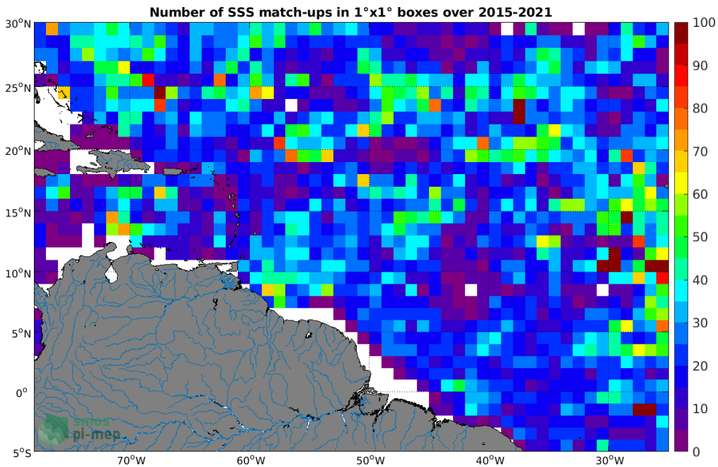
Figure 4: Number of SSS match-ups between Argo SSS and the SMAP SSS L3 v4 - Monthly (RSS) SSS product for the Amazon and Orinoco river plumes Pi-MEP region over 1^\circ \times 1^\circ boxes and for the full satellite product period.
