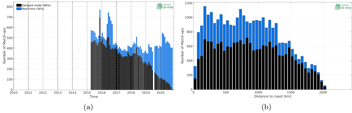
Figure 1: Number of match-ups between Argo and SMAP SSS L3 v4 - Monthly (RSS) SSS as a function of time (a) and as function of the distance to coast (b) over the Amazon and Orinoco river plumes Pi-MEP region and for the full satellite product period.
