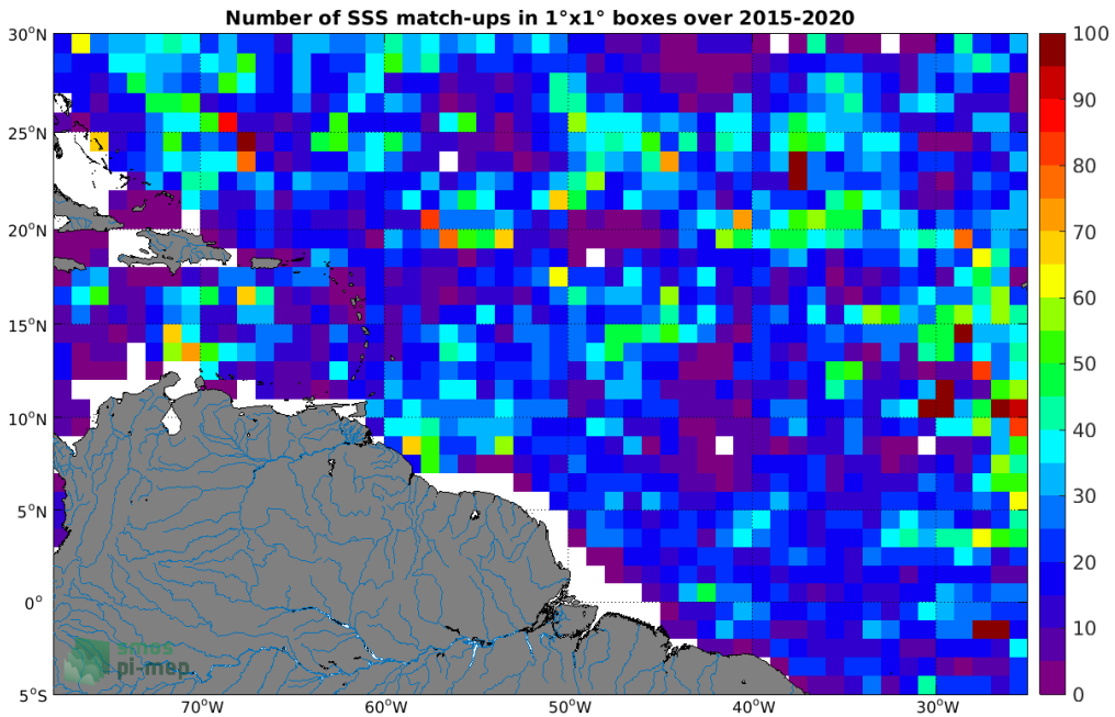
Figure 4: Number of SSS match-ups between Argo SSS and the SMAP SSS L3 v4 - Monthly (RSS) SSS product for the Amazon and Orinoco river plumes Pi-MEP region over 1°x1° boxes and for the full satellite product period.
