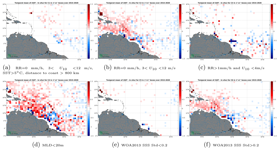
Figure 12: Temporal mean gridded over spatial boxes of size 1°x1° of \Delta SSS (SMAP SSS L3 v4 - Monthly (RSS) - Argo) for 6 different subdatasets corresponding to:RR=0 mm/h, 3 < U_{10} < 12 m/s, SST>5°C, distance to coast > 800 km (a), RR=0 mm/h, 3 < U_{10} < 12 m/s (b), RR>1mm/h and U_{10} < 4 m/s (c),MLD<20m (d),WOA2013 SSS Std<0.2 (e),WOA2013 SSS Std>0.2 (f).
