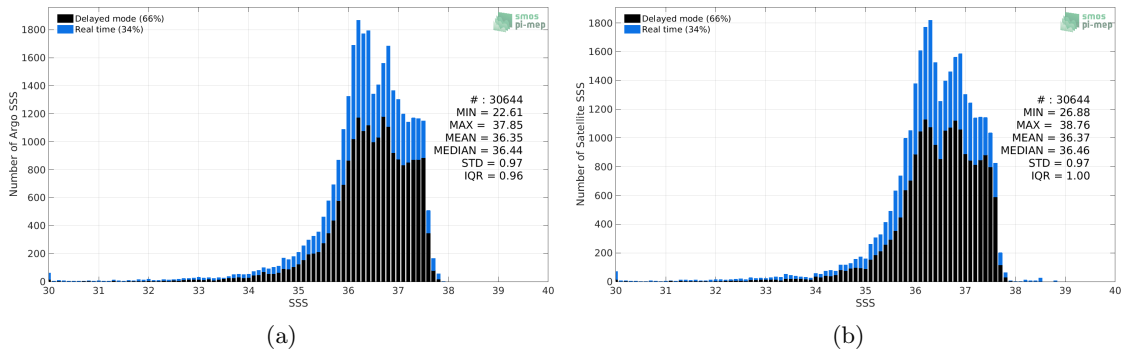
Figure 2: Histograms of SSS from Argo (a) and SMAP SSS L3 v4 - Monthly (RSS) (b) considering all match-up pairs per bins of 0.1 over the Amazon and Orinoco river plumes Pi-MEP region and for the full satellite product period.
