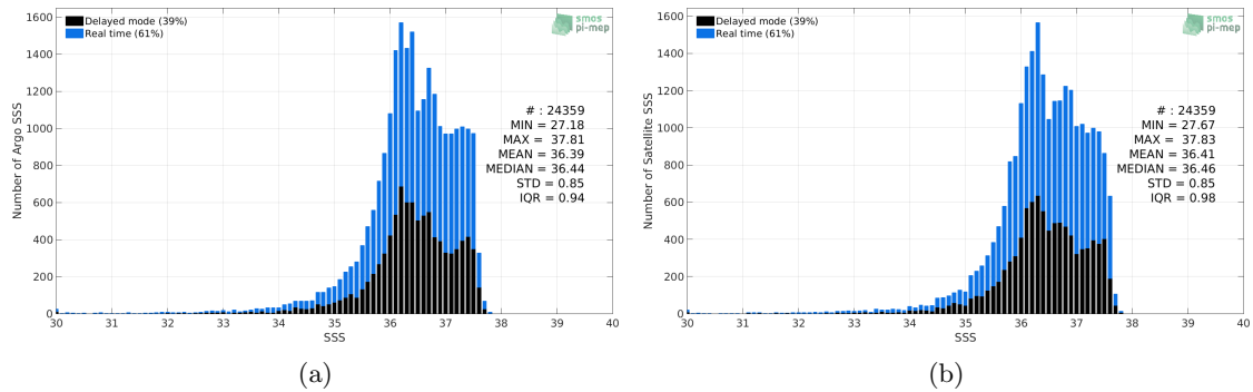
Figure 2: Histograms of SSS from Argo (a) and SMAP-L3-RSS-V4-MONTHLY (b) considering all match-up pairs per bins of 0.1 over the Amazon and Orinoco river plumes Pi-MEP region and for the full satellite product period.
