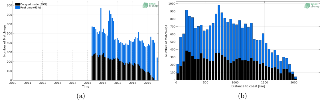
Figure 1: Number of match-ups between Argo and SMAP-L3-RSS-V4-MONTHLY SSS as a function of time (a) and as function of the distance to coast (b) over the Amazon and Orinoco river plumes Pi-MEP region and for the full satellite product period.
