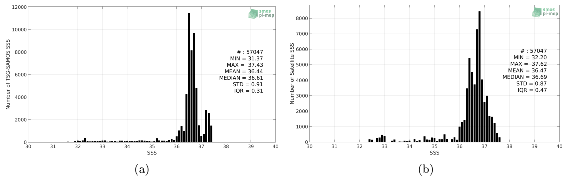
Figure 2: Histograms of SSS from TSG-SAMOS (a) and SMAP-L3-RSS-V3-8DAY-RUNNING-70KM (b) considering all match-up pairs per bins of 0.1 over the Amazon and Orinoco river plumes Pi-MEP region and for the full satellite product period.
