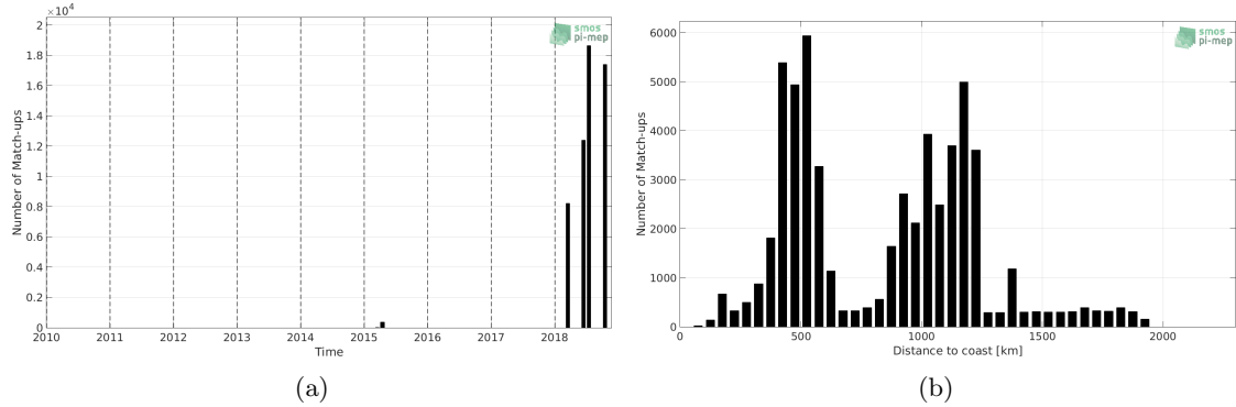
Figure 1: Number of match-ups between TSG-SAMOS and SMAP-L3-RSS-V3-8DAY-RUNNING-70KM SSS as a function of time (a) and as function of the distance to coast (b) over the Amazon and Orinoco river plumes Pi-MEP region and for the full satellite product period.
