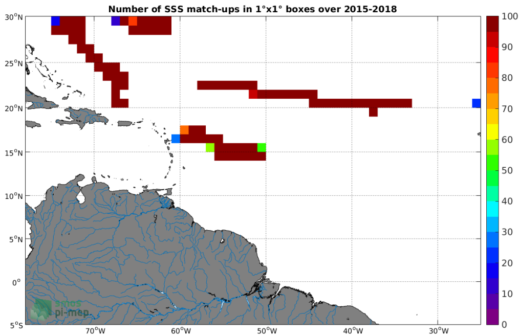
Figure 4: Number of SSS match-ups between TSG-SAMOS SSS and the SMAP-L3-RSS-V3-8DAY-RUNNING-70KM SSS product for the Amazon and Orinoco river plumes Pi-MEP region over 1^\circ \times 1^\circ boxes and for the full satellite product period.
