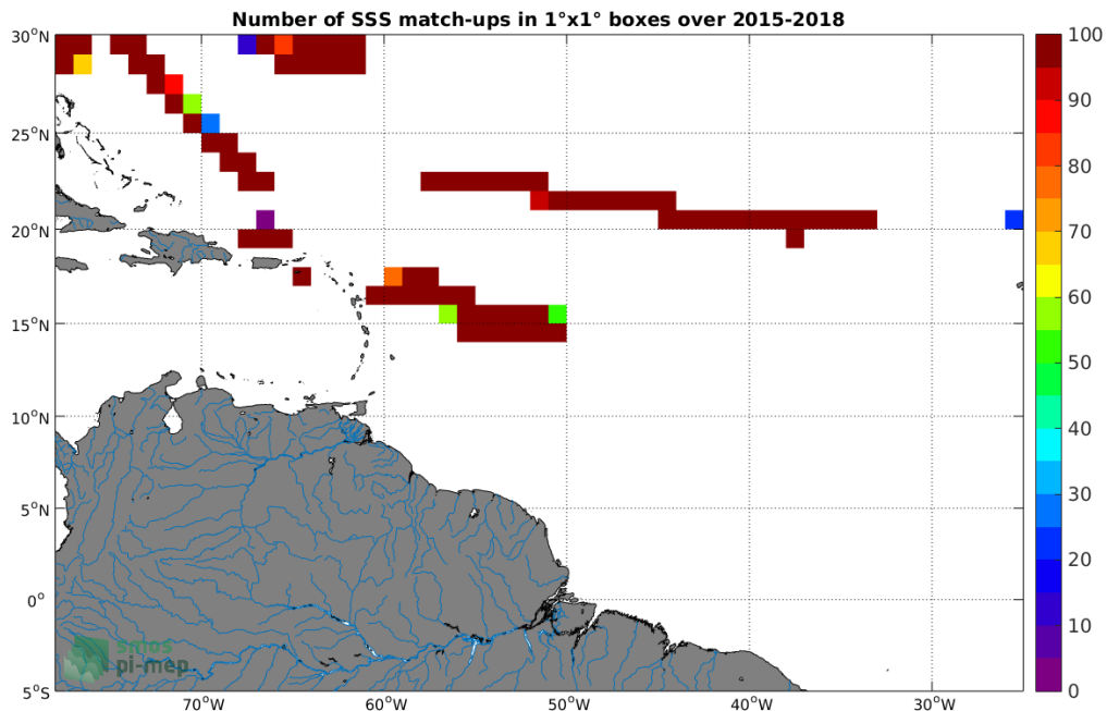
Figure 4: Number of SSS match-ups between TSG-SAMOS SSS and the SMAP-L3-RSS-V3-8DAY-RUNNING-70KM SSS product for the Amazon and Orinoco river plumes Pi-MEP region over 1°x1° boxes and for the full satellite product period.
