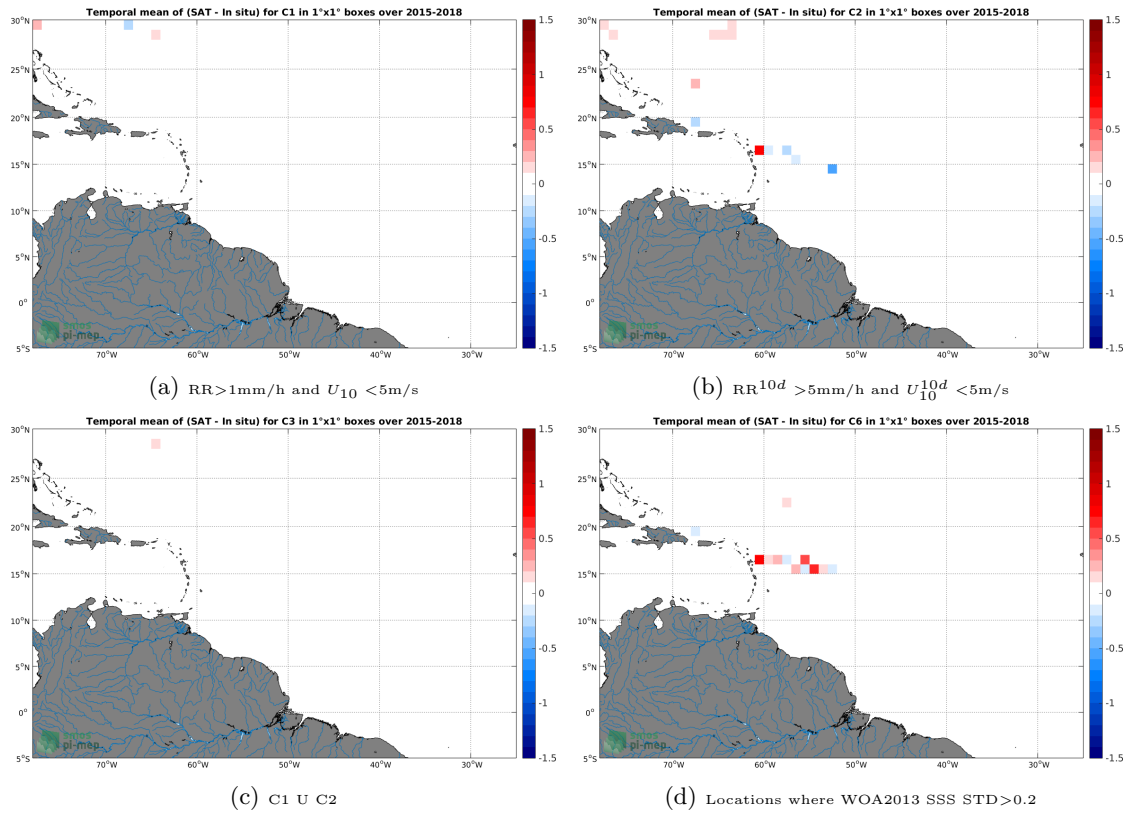
Figure 12: Temporal mean gridded over spatial boxes of size 1^\circ \times 1^\circ of \Delta SSS (SMAP-L3-RSS-V3-8DAY-RUNNING-70KM - TSG-SAMOS) for 4 different subdatasets corresponding to: RR > 1mm/h and U_{10} < 5\text{m/s} (a), RR^{10d} > 5\text{mm/h} and U_{10}^{10d} < 5\text{m/s} (b), C1 U C2 (c), Locations where WOA2013 SSS STD > 0.2 (d).
