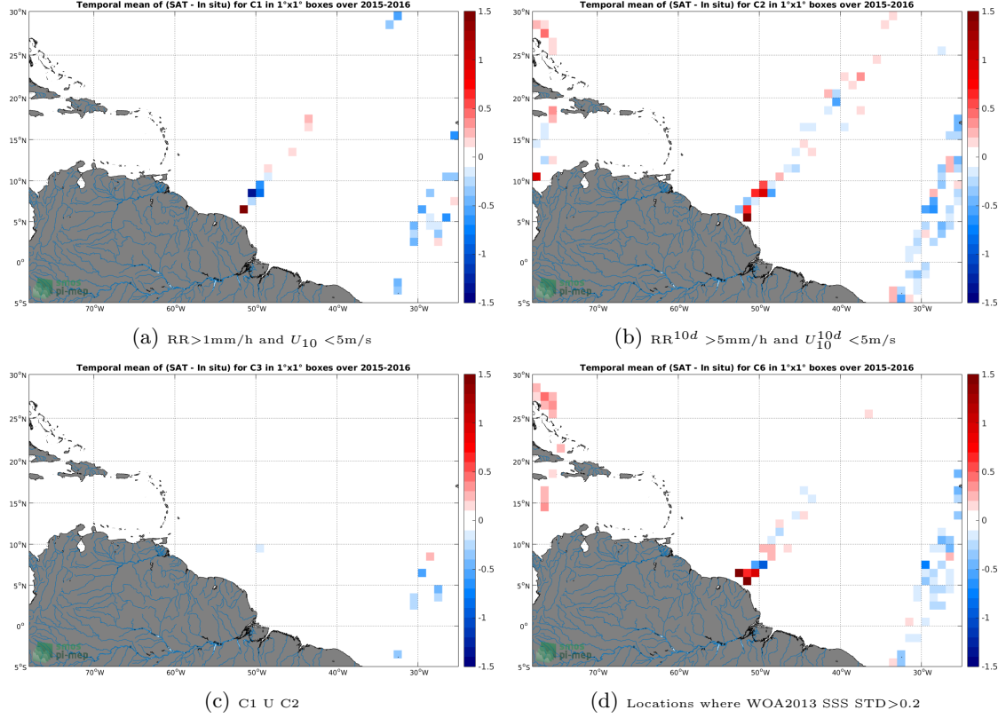
Figure 12: Temporal mean gridded over spatial boxes of size 1^\circ \times 1^\circ of \Delta SSS (SMAP-L3-RSS-V3-8DAY-RUNNING-70KM - TSG-LEGOS-DM) for 4 different subdatasets corresponding to: RR > 1\text{mm/h} and U_{10} < 5\text{m/s} (a), RR^{10d} > 5\text{mm/h} and U_{10}^{10d} < 5\text{m/s} (b), C1 U C2 (c), Locations where WOA2013 SSS STD > 0.2 (d).
