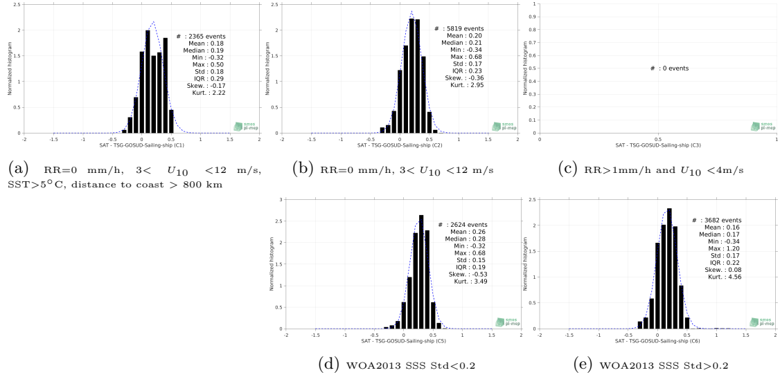
Figure 13: Normalized histogram of \Delta SSS (SMAP-L3-RSS-V3-8DAY-RUNNING-70KM - TSG-GOSUD-Sailing-ship) for 5 different subdatasets corresponding to: RR=0 mm/h, 3 < U_{10} < 12 m/s, SST > 5°C, distance to coast > 800 km (a), RR=0 mm/h, 3 < U_{10} < 12 m/s (b), RR > 1mm/h and U_{10} < 4 m/s (c), WOA2013 SSS Std < 0.2 (d), WOA2013 SSS Std > 0.2 (e).
