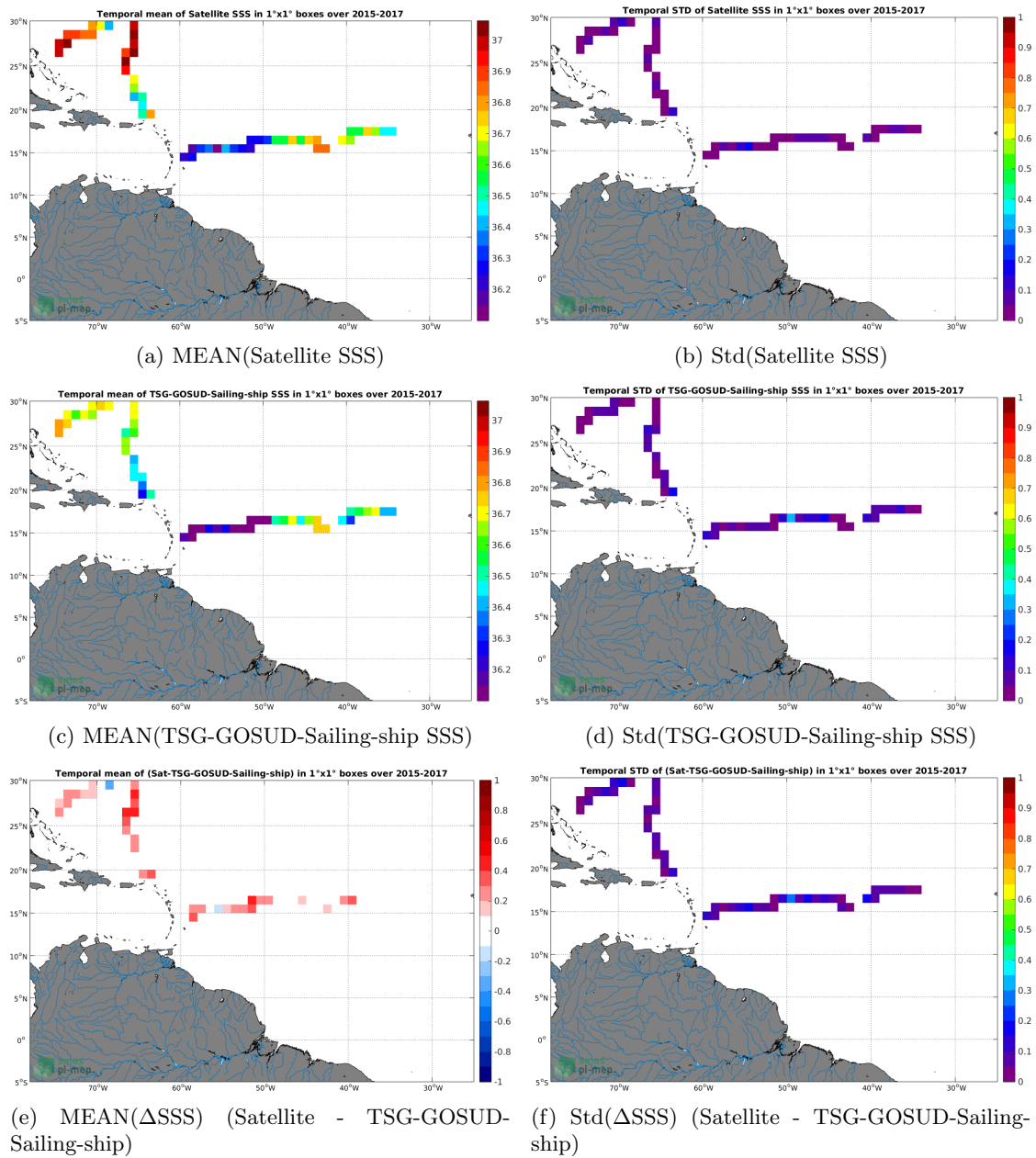
Figure 6: Temporal mean (left) and Std (right) of SSS from SMAP-L3-RSS-V3-8DAY-RUNNING-70KM (top), TSG-GOSUD-Sailing-ship (middle), and of \Delta SSS (Satellite - TSG-GOSUD-Sailing-ship). Only match-up pairs are used to generate these maps.
