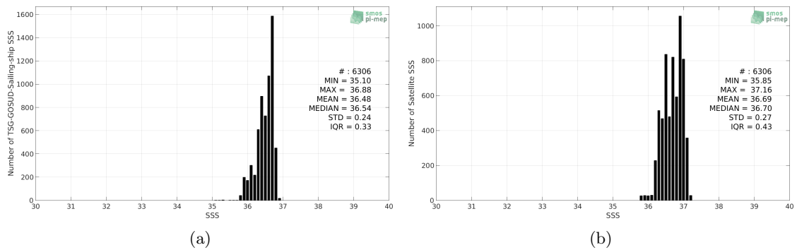
Figure 2: Histograms of SSS from TSG-GOSUD-Sailing-ship (a) and SMAP-L3-RSS-V3-8DAY-RUNNING-70KM (b) considering all match-up pairs per bins of 0.1 over the Amazon and Orinoco river plumes Pi-MEP region and for the full satellite product period.
