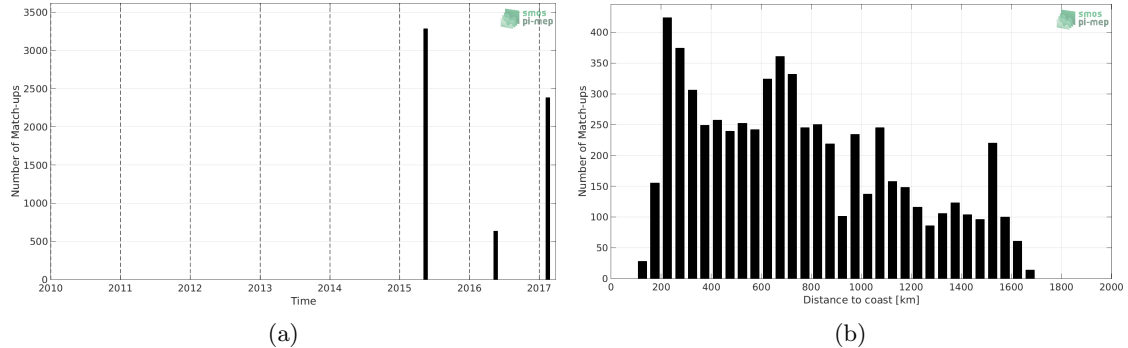
Figure 1: Number of match-ups between TSG-GOSUD-Sailing-ship and SMAP-L3-RSS-V3-8DAY-RUNNING-70KM SSS as a function of time (a) and as function of the distance to coast (b) over the Amazon and Orinoco river plumes Pi-MEP region and for the full satellite product period.
