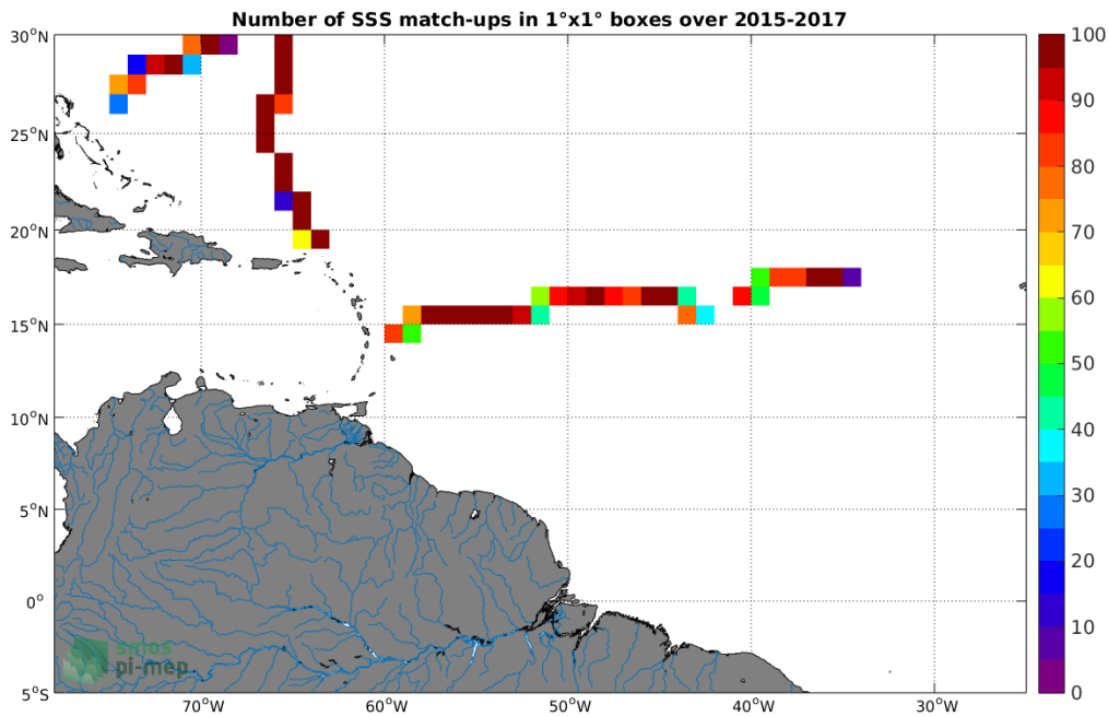
Figure 4: Number of SSS match-ups between TSG-GOSUD-Sailing-ship SSS and the SMAP-L3-RSS-V3-8DAY-RUNNING-70KM SSS product for the Amazon and Orinoco river plumes Pi-MEP region over 1°x1° boxes and for the full satellite product period.
