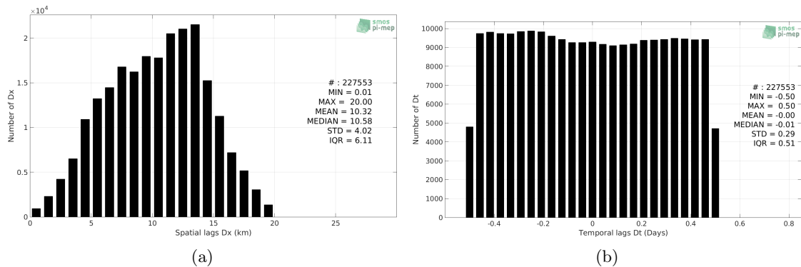
Figure 5: Histograms of the spatial (a) and temporal (b) lags between the time of the TSG-GOSUD-Research-vessel measurements and the date of the corresponding SMAP-L3-RSS-V3-8DAY-RUNNING-40KM SSS product.
