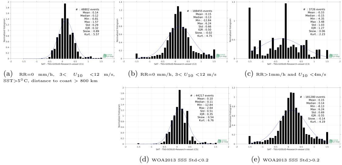
Figure 13: Normalized histogram of \Delta SSS (SMAP-L3-RSS-V3-8DAY-RUNNING-40KM - TSG-GOSUD-Research-vessel) for 5 different subdatasets corresponding to: RR=0 mm/h, 3 < U_{10} < 12 m/s, SST>5°C, distance to coast > 800 km (a), RR=0 mm/h, 3 < U_{10} < 12 m/s (b), RR>1mm/h and U_{10} < 4 m/s (c), WOA2013 SSS Std<0.2 (d), WOA2013 SSS Std>0.2 (e).
