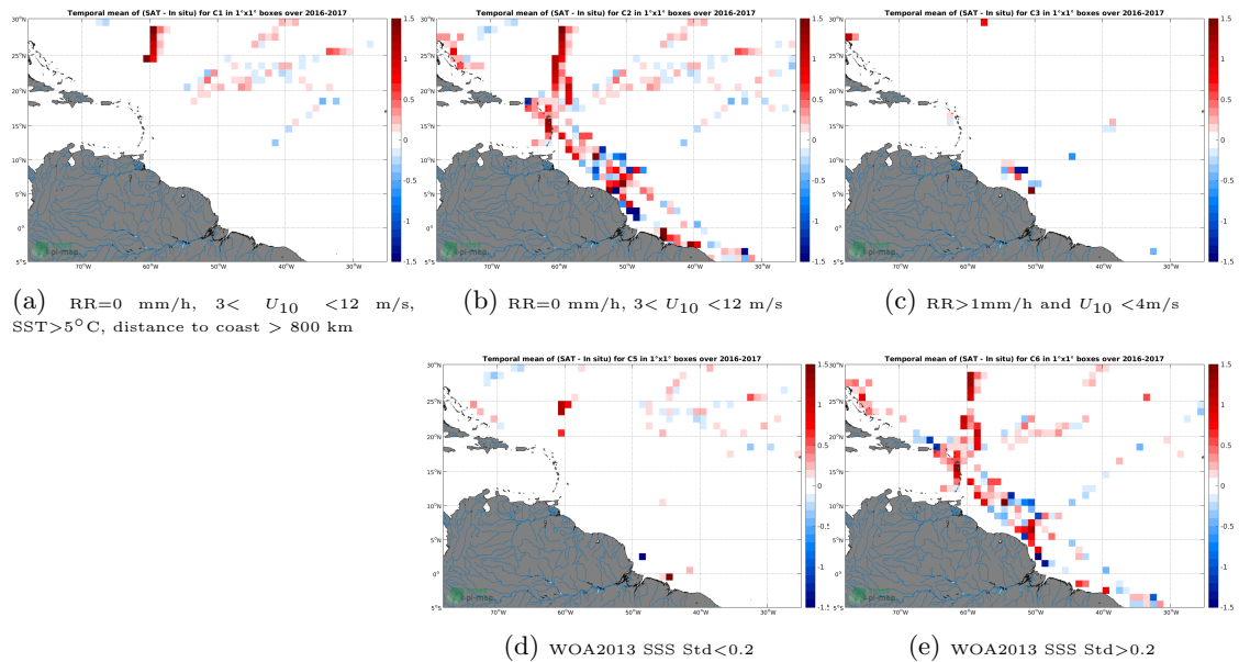
Figure 12: Temporal mean gridded over spatial boxes of size 1^\circ \times 1^\circ of \Delta SSS (SMAP-L3-RSS-V3-8DAY-RUNNING-40KM - TSG-GOSUD-Research-vessel) for 5 different subdatasets corresponding to:RR=0 mm/h, 3 < U_{10} < 12 m/s, SST > 5^\circ\text{C} , distance to coast > 800 km (a), RR=0 mm/h, 3 < U_{10} < 12 m/s (b), RR > 1 mm/h and U_{10} < 4 m/s (c), WOA2013 SSS Std < 0.2 (d), WOA2013 SSS Std > 0.2 (e).
