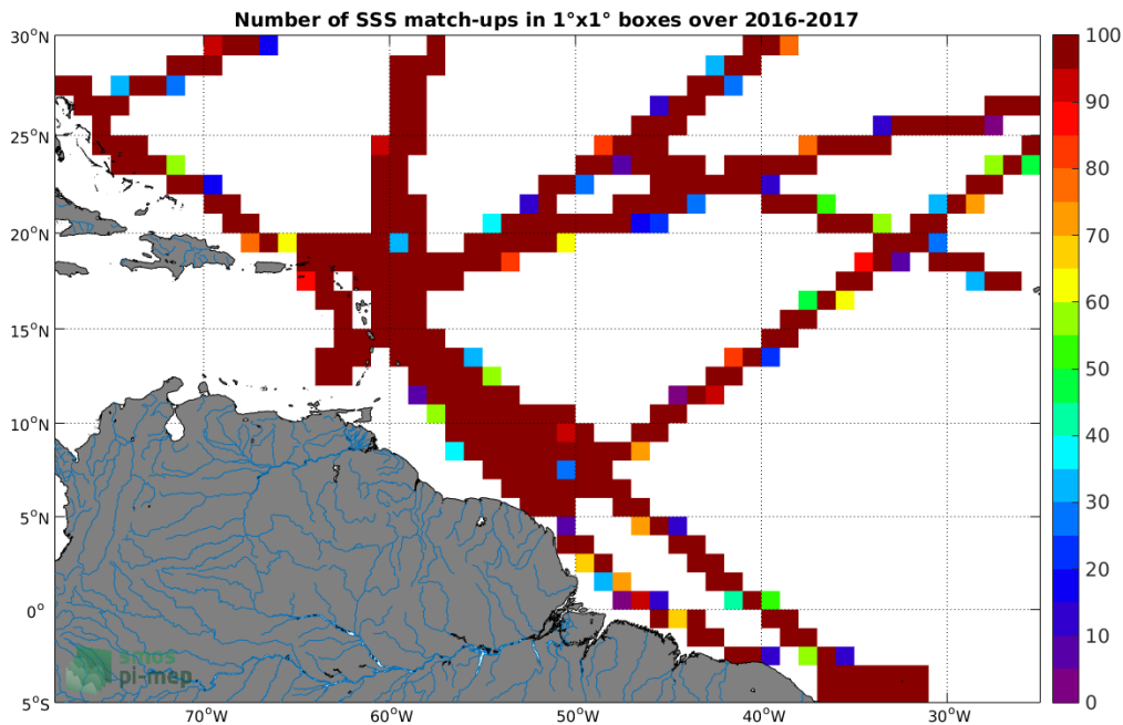
Figure 4: Number of SSS match-ups between TSG-GOSUD-Research-vessel SSS and the SMAP-L3-RSS-V3-8DAY-RUNNING-40KM SSS product for the Amazon and Orinoco river plumes Pi-MEP region over 1^\circ \times 1^\circ boxes and for the full satellite product period.
