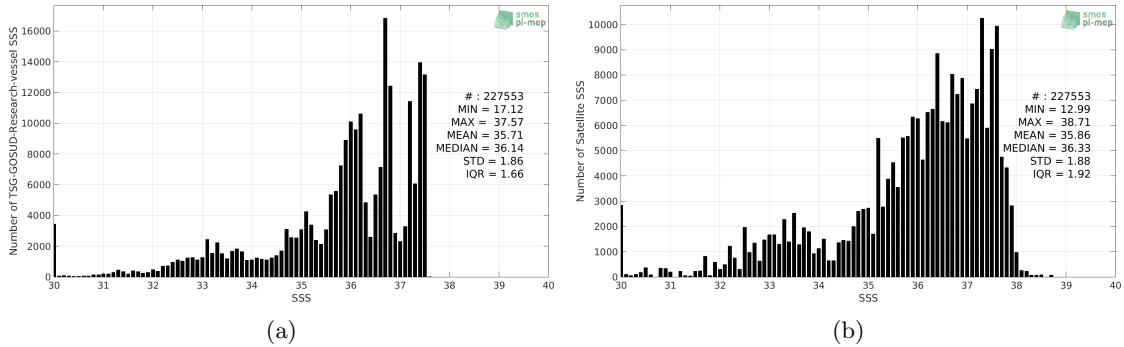
Figure 2: Histograms of SSS from TSG-GOSUD-Research-vessel (a) and SMAP-L3-RSS-V3-8DAY-RUNNING-40KM (b) considering all match-up pairs per bins of 0.1 over the Amazon and Orinoco river plumes Pi-MEP region and for the full satellite product period.
