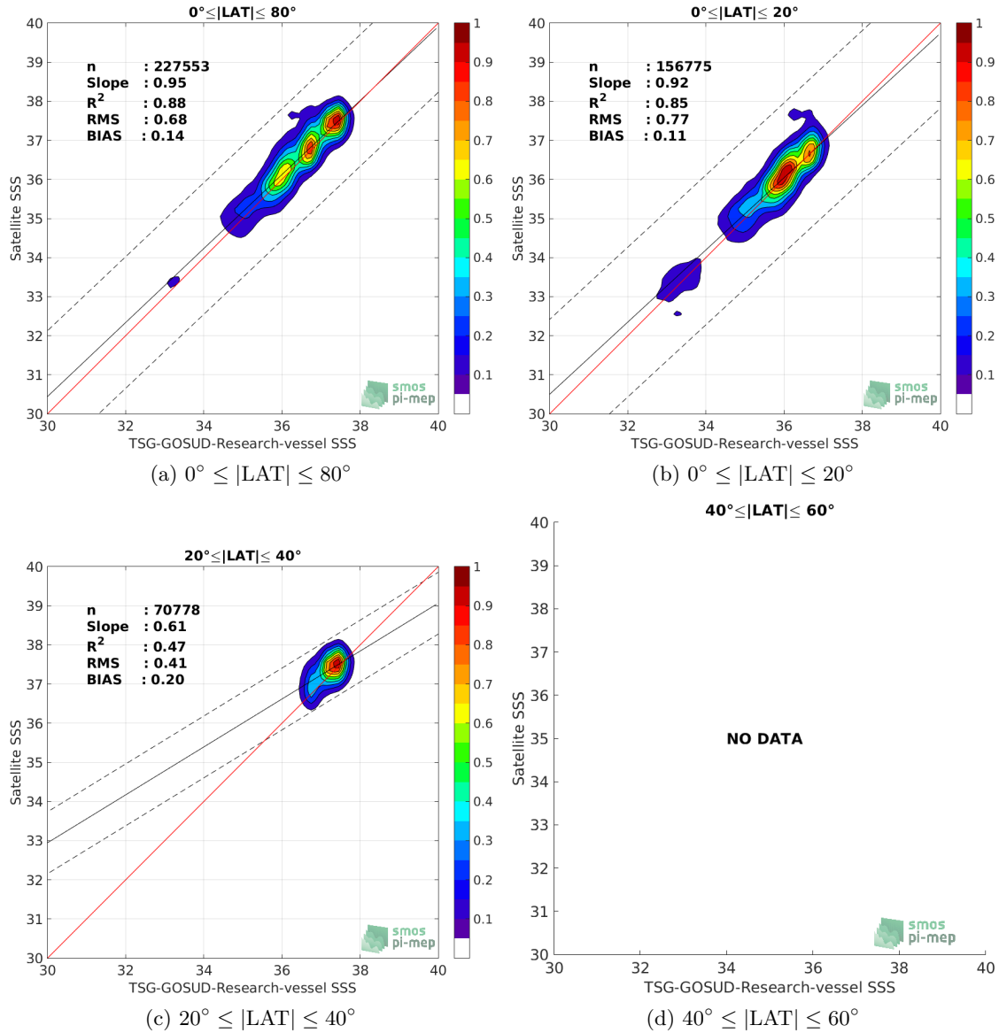
Figure 9: Contour maps of the concentration of SMAP-L3-RSS-V3-8DAY-RUNNING-40KM SSS (y-axis) versus TSG-GOSUD-Research-vessel SSS (x-axis) at match-up pairs for different latitude bands. For each plot, the red line shows x=y . The black thin and dashed lines indicate a linear fit through the data cloud and the \pm 95\% confidence levels, respectively. The number match-up pairs n , the slope and R^2 coefficient of the linear fit, the root mean square (RMS) and the mean bias between satellite and in situ data are indicated for each latitude band in each plots.
