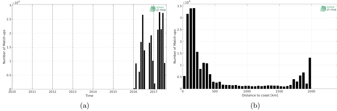
Figure 1: Number of match-ups between TSG-GOSUD-Research-vessel and SMAP-L3-RSS-V3-8DAY-RUNNING-40KM SSS as a function of time (a) and as function of the distance to coast (b) over the Amazon and Orinoco river plumes Pi-MEP region and for the full satellite product period.
