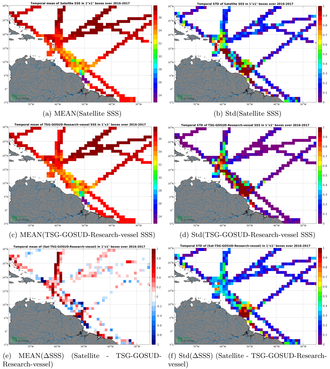
Figure 6: Temporal mean (left) and Std (right) of SSS from SMAP-L3-RSS-V3-8DAY-RUNNING-40KM (top), TSG-GOSUD-Research-vessel (middle), and of \Delta SSS (Satellite - TSG-GOSUD-Research-vessel). Only match-up pairs are used to generate these maps.
