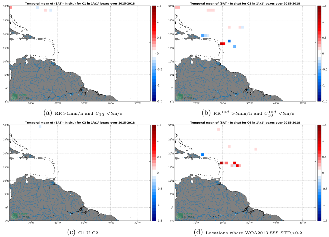
Figure 12: Temporal mean gridded over spatial boxes of size 1^\circ \times 1^\circ of \Delta SSS (SMAP-L3-RSS-V3-MONTHLY-70KM - TSG-SAMOS) for 4 different subdatasets corresponding to: RR > 1\text{mm/h} and U_{10} < 5\text{m/s} (a), RR^{10d} > 5\text{mm/h} and U_{10}^{10d} < 5\text{m/s} (b), C1 U C2 (c), Locations where WOA2013 SSS STD > 0.2 (d).
