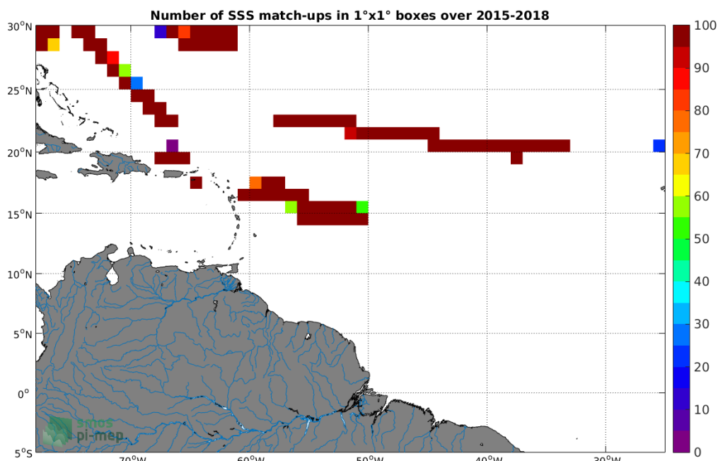
Figure 4: Number of SSS match-ups between TSG-SAMOS SSS and the SMAP-L3-RSS-V3-MONTHLY-70KM SSS product for the Amazon and Orinoco river plumes Pi-MEP region over 1°x1° boxes and for the full satellite product period.
