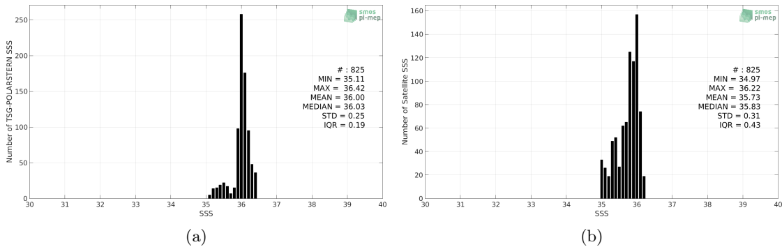
Figure 2: Histograms of SSS from TSG-POLARSTERN (a) and SMAP-L3-RSS-V3-MONTHLY-70KM (b) considering all match-up pairs per bins of 0.1 over the Amazon and Orinoco river plumes Pi-MEP region and for the full satellite product period.
