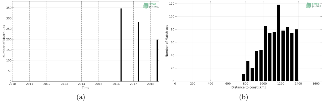
Figure 1: Number of match-ups between TSG-POLARSTERN and SMAP-L3-RSS-V3-MONTHLY-70KM SSS as a function of time (a) and as function of the distance to coast (b) over the Amazon and Orinoco river plumes Pi-MEP region and for the full satellite product period.
