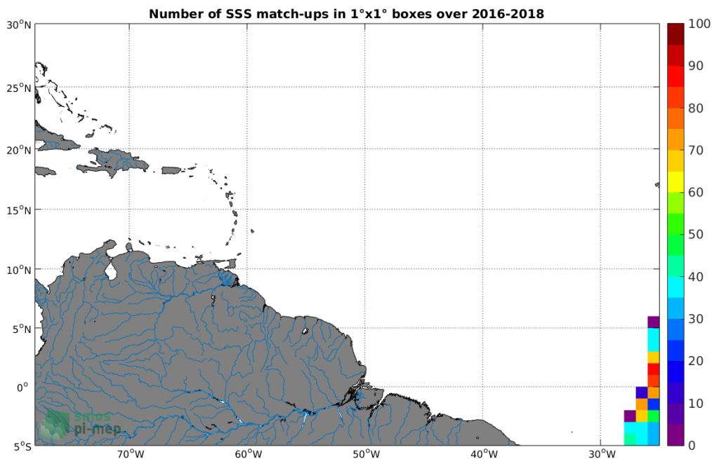
Figure 4: Number of SSS match-ups between TSG-POLARSTERN SSS and the SMAP-L3-RSS-V3-MONTHLY-70KM SSS product for the Amazon and Orinoco river plumes Pi-MEP region over 1^\circ \times 1^\circ boxes and for the full satellite product period.
